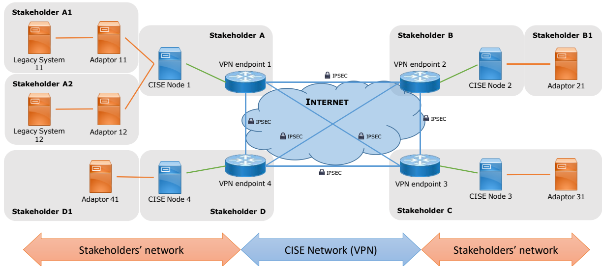
Figure 18. The network between CISE Nodes, including adaptors and legacy systems.
