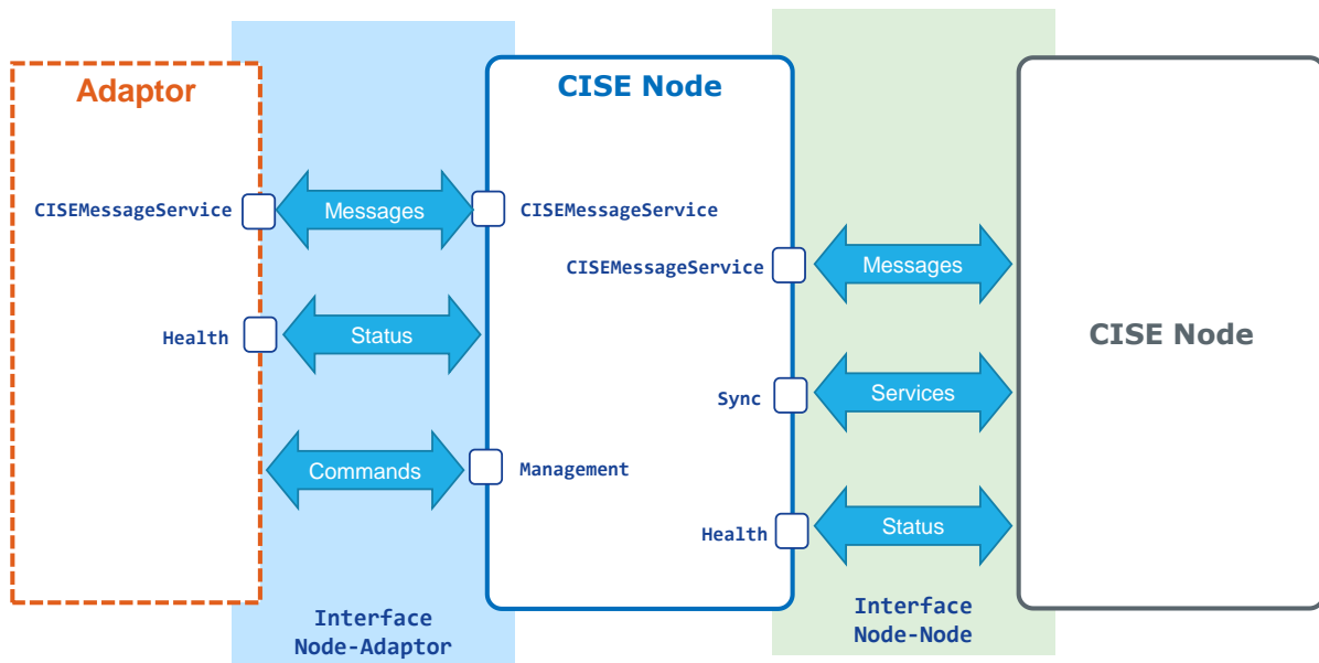
Figure 16. External interfaces of the CISE Node.
