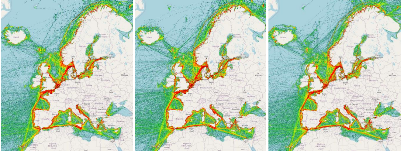
Figure 8: All ship types: ship traffic density in December 2019 (left), in December 2020 (centre) and in December 2021 (right)
