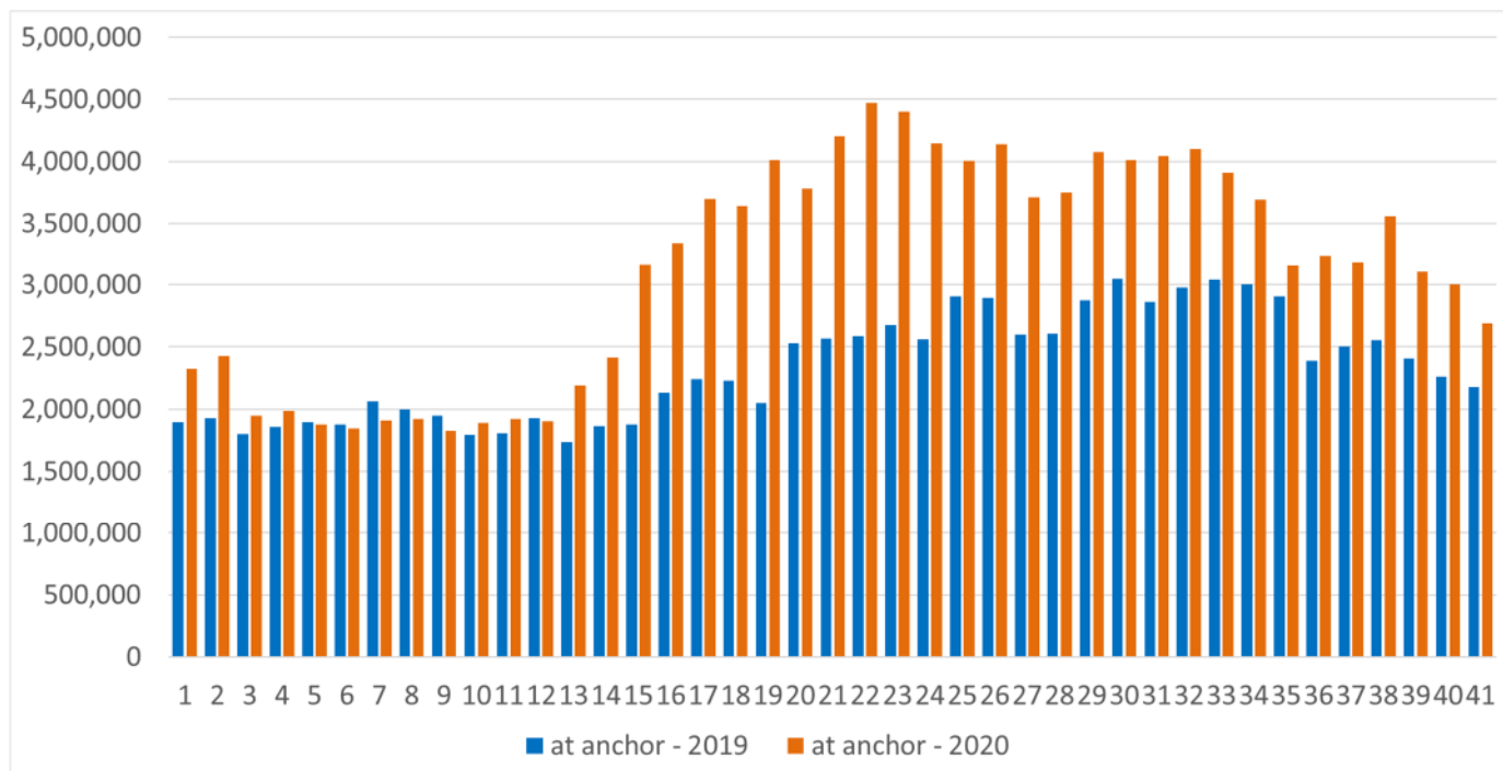
Figure 11: AIS data reports reporting navigational status “at anchor” in and around EU waters in 2019 and 2020 (weeks 1 to 41)
