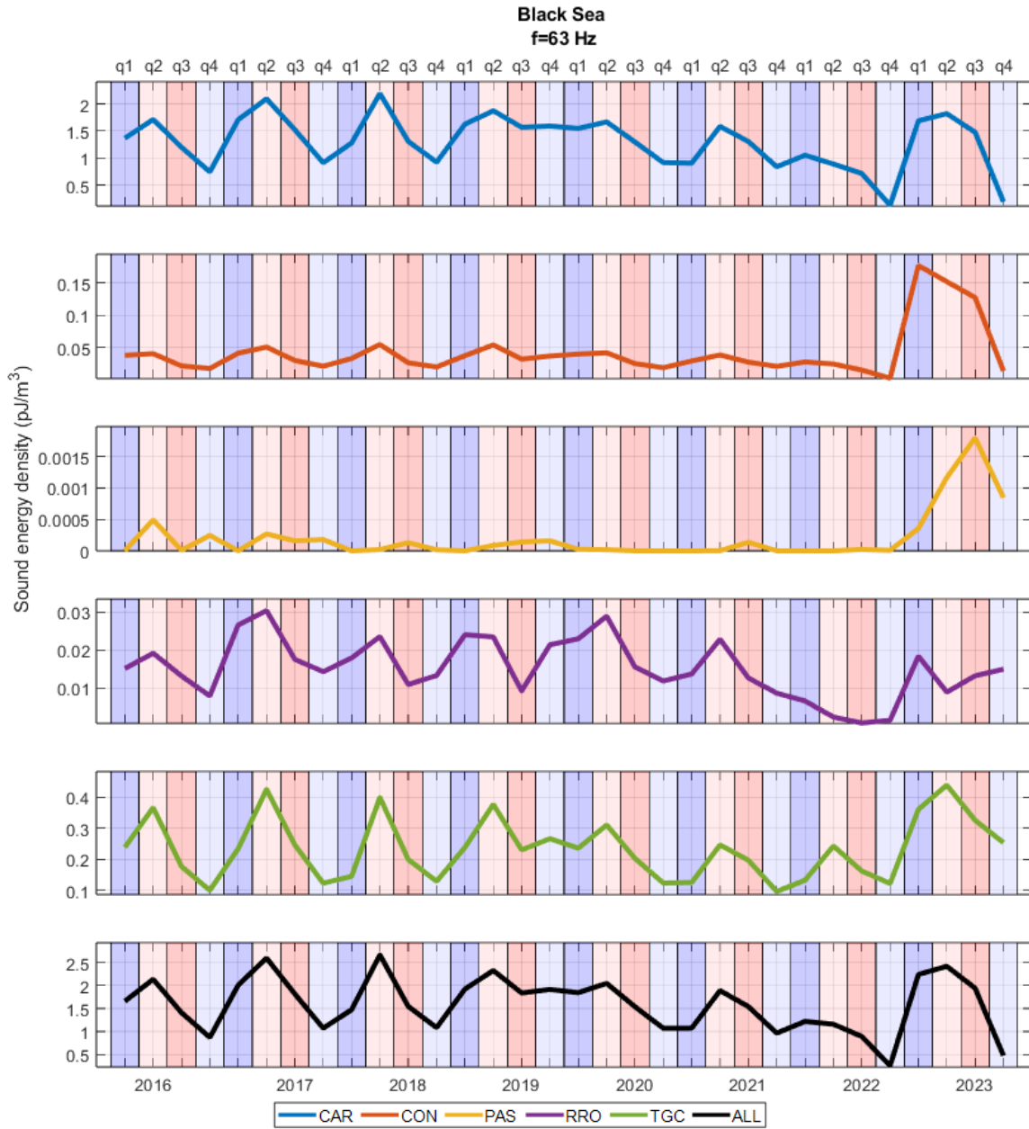
Figure 30 Black Sea: Sound energy density (in pJ/m 3 ) of different vessel categories for each quarter in chronological order at 63 Hz.
