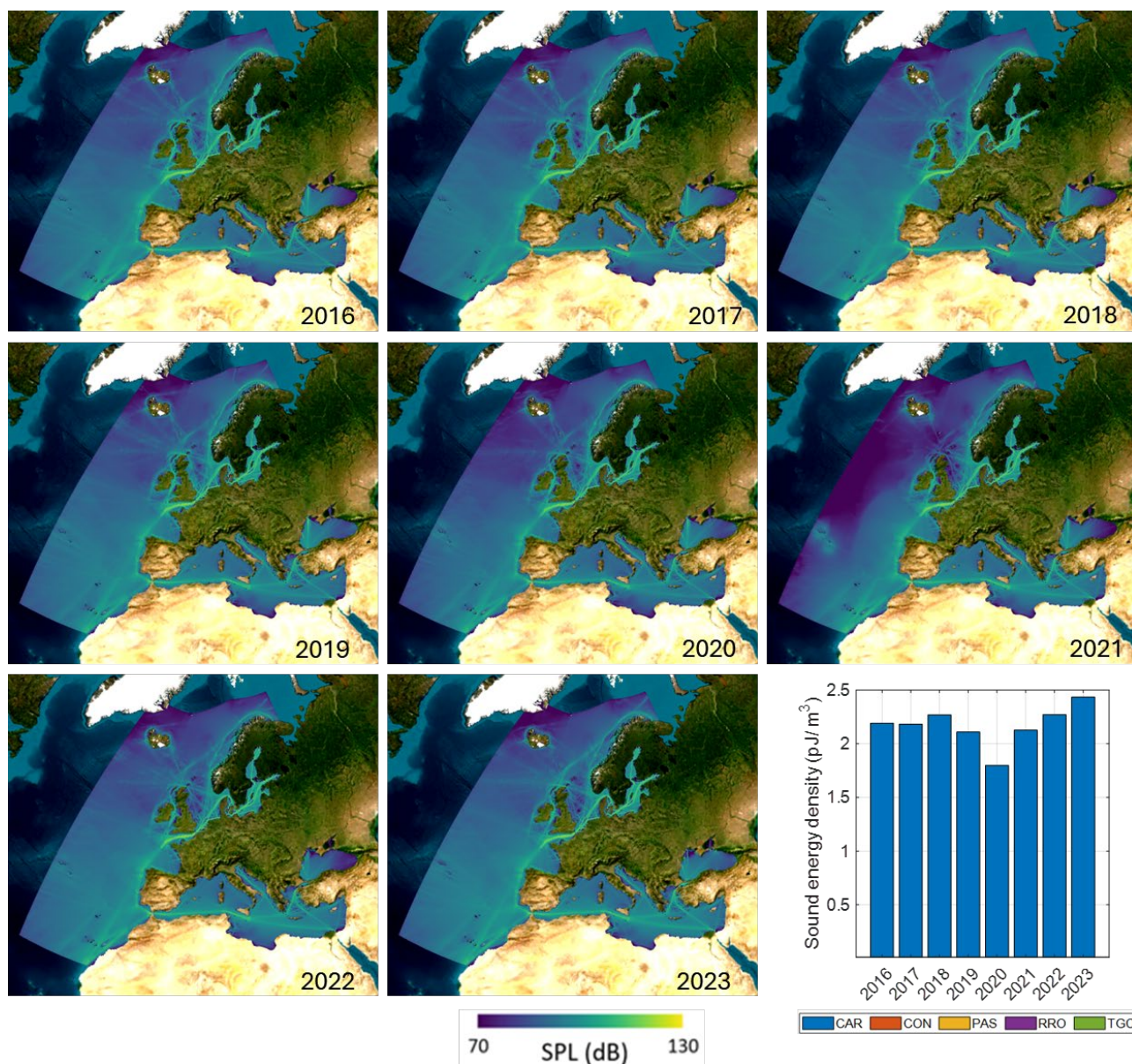
Figure 10 CAR vessel categories: Annually averaged sound map layers (SPL re 1 \mu Pa, in dB) including sound energy density (in pJ/m 3 ) at 63 Hz. One picojoule (1 pJ) is equal to one trillionth of a joule ( 10^{-12} J).
