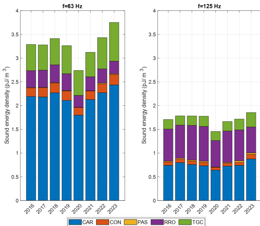
Figure 16 Europe: Annually averaged sound energy density (in pJ/m³) at (left) 63 Hz and (right) 125 Hz.
