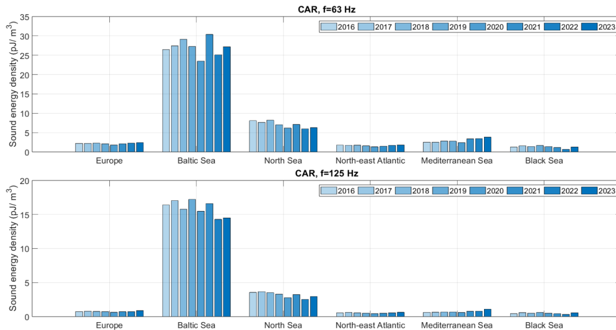
Figure 49 CAR vessels: Sound energy density (in \text{pJ}/\text{m}^3 ) in different regions at (top) 63 Hz and (bottom) 125 Hz.
