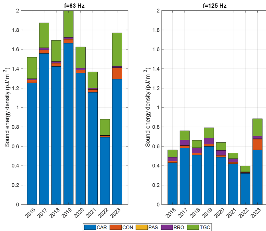
Figure 28 Black Sea: Annually averaged sound energy density (in \text{pJ}/\text{m}^3 ) at (left) 63 Hz and (right) 125 Hz.
