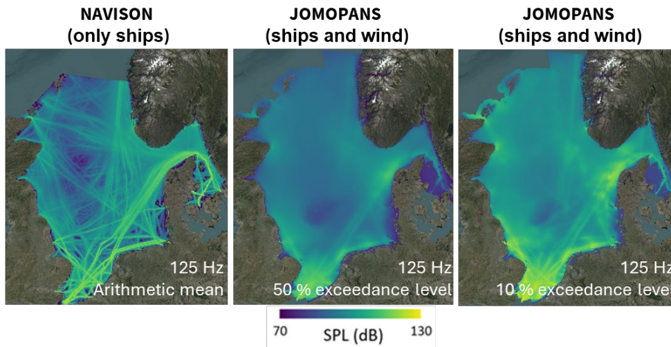
Figure 96 Comparison between (left) NAVISION (only ships) and (right) JOMOPANS (ships and wind) sound maps (SPL re 1 \mu\text{Pa}^2 , in dB) at 125 Hz. The NAVISION results are based on spatially averaged sound pressure level while the JOMOPANS results are for 50 and 10 % exceedance levels.
