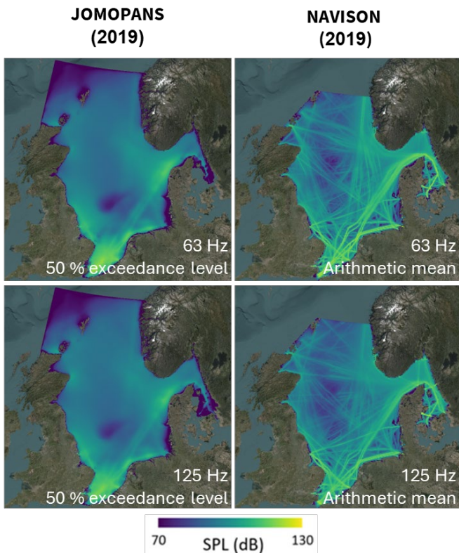
Figure 95 Comparison between (left) JOMOPANS and (right) NAVISON and sound maps (SPL re 1 μPa 2 , in dB) at (top) 63 Hz and (bottom) 125 Hz. The NAVISON results are based on spatially averaged sound pressure level while the JOMOPANS results are for the median (temporal 50 % exceedance level of depth-averaged sound pressure level). See Table 8 for detailed description of the metrics for each project.
