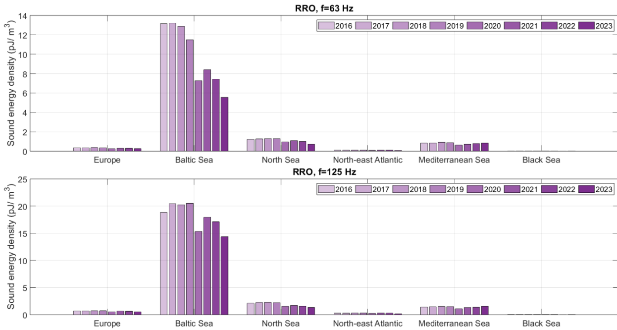
Figure 52 RRO vessels: Sound energy density (in pJ/m 3 ) in different regions at (top) 63 Hz and (bottom) 125 Hz.
