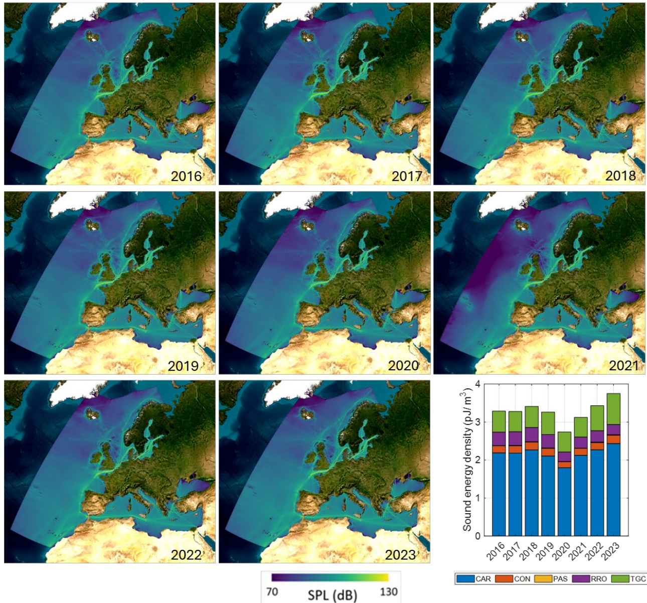
Figure 9 ALL vessel categories: Annually averaged sound map layers (SPL re 1 \mu\text{Pa}^2 , in dB) including sound energy density (in \text{pJ}/\text{m}^3 ) at 63 Hz. One picojoule (1 pJ) is equal to one trillionth of a joule ( 10^{-12} J).
