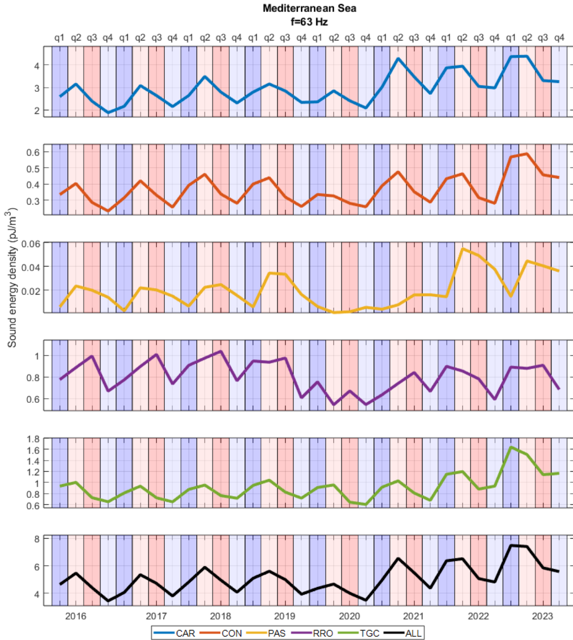
Figure 37 Mediterranean Sea: Sound energy density (in pJ/m³) of different vessel categories for each quarter in chronological order for 63 Hz.
