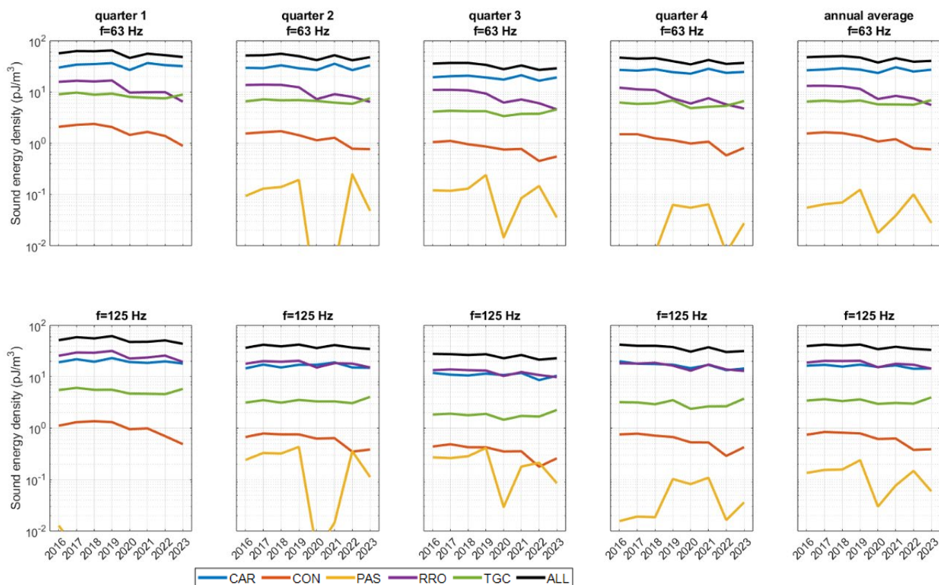
Figure 24 Baltic Sea: Sound energy density (in pJ/m 3 ) of different vessel categories for each quarter and year for (top) 63 Hz and (bottom) 125 Hz.
