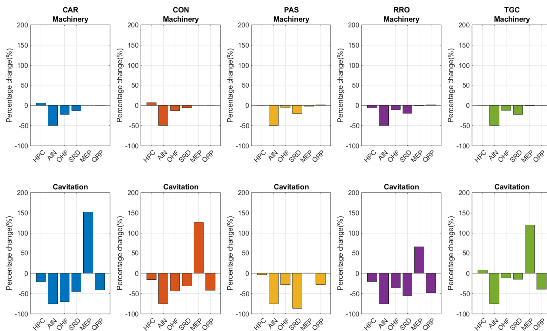
Figure 75 North Sea: Forecast percentage change in the sound energy density for (top) machinery and (bottom) cavitation components compared to the BAU scenario at 63 Hz.
