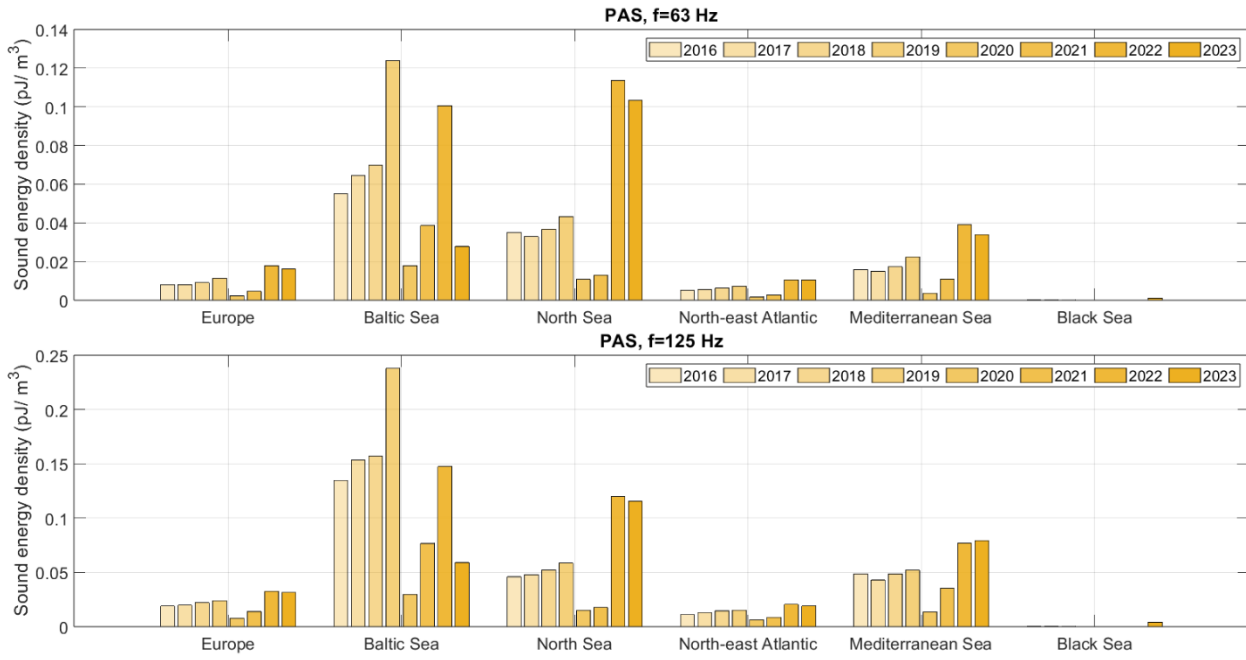
Figure 51 PAS vessels: Sound energy density (in pJ/m 3 ) in different regions at (top) 63 Hz and (bottom) 125 Hz
