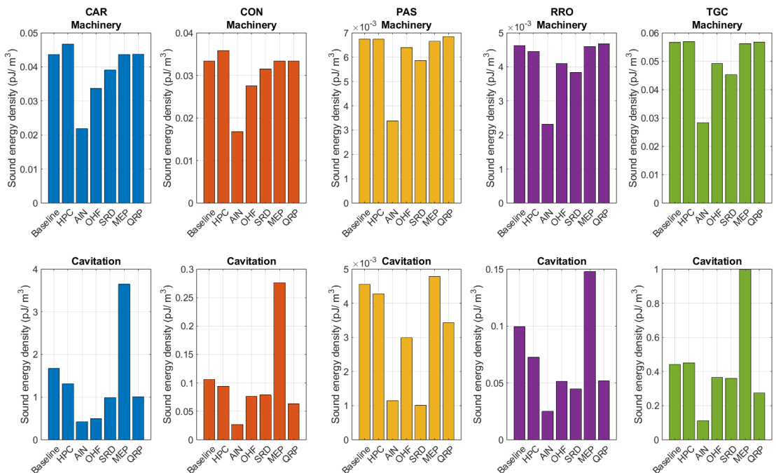
Figure 78 Northeast Atlantic Ocean: Forecast sound energy density for the 100 % penetration rates for each mitigation measure at 63 Hz. Sound energy density is calculated for (top) machinery and (bottom) cavitation components.
