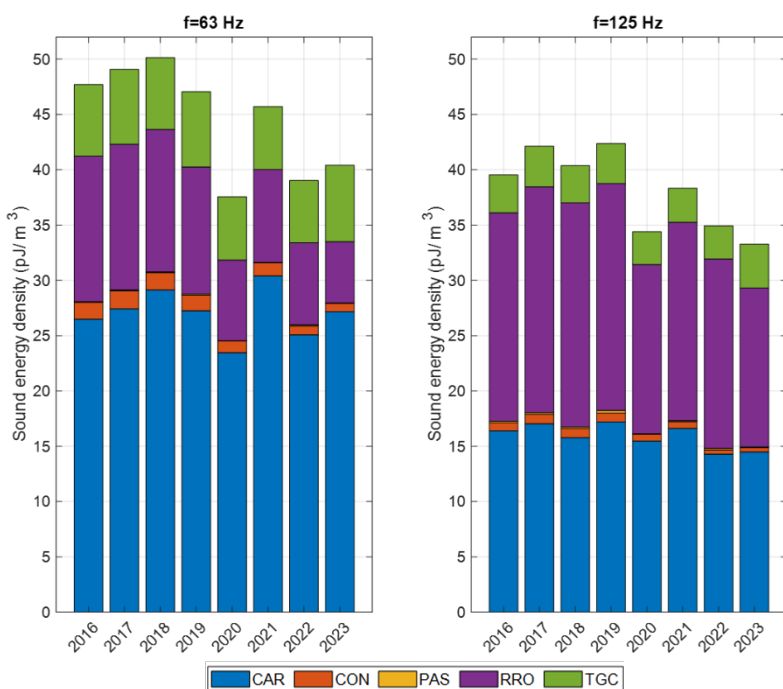
Figure 23 Baltic Sea: Annually averaged sound energy density (in pJ/m³) at (left) 63 Hz and (right) 125 Hz.
