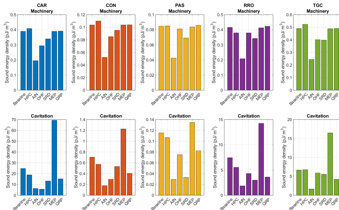
Figure 62 Baltic Sea: Forecast sound energy density for the 100 % penetration rates for each mitigation measure at 63 Hz. Sound energy density is calculated for (top) machinery and (bottom) cavitation components.
