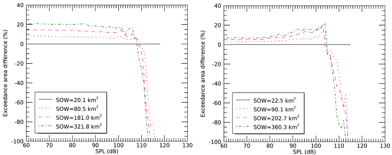
Figure 92 Percentage difference in exceedance area versus underwater noise limit value (UNLV) in the (left) Baltic Sea and (right) North Sea for different sizes of spatial observation window (SOW).
