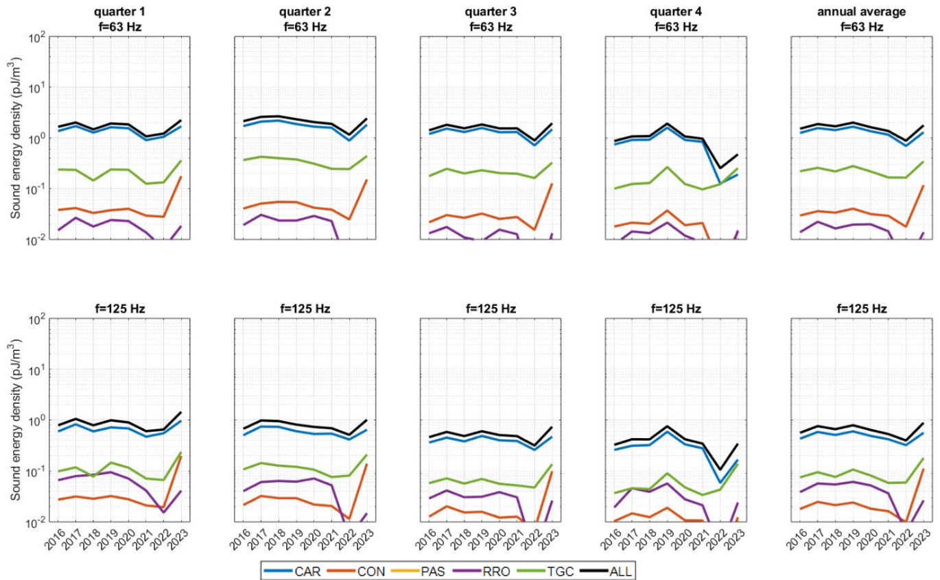
Figure 29 Black Sea: Sound energy density (in \text{pJ/m}^3 ) of different vessel categories for each quarter and year for (top) 63 Hz and (bottom) 125 Hz.
