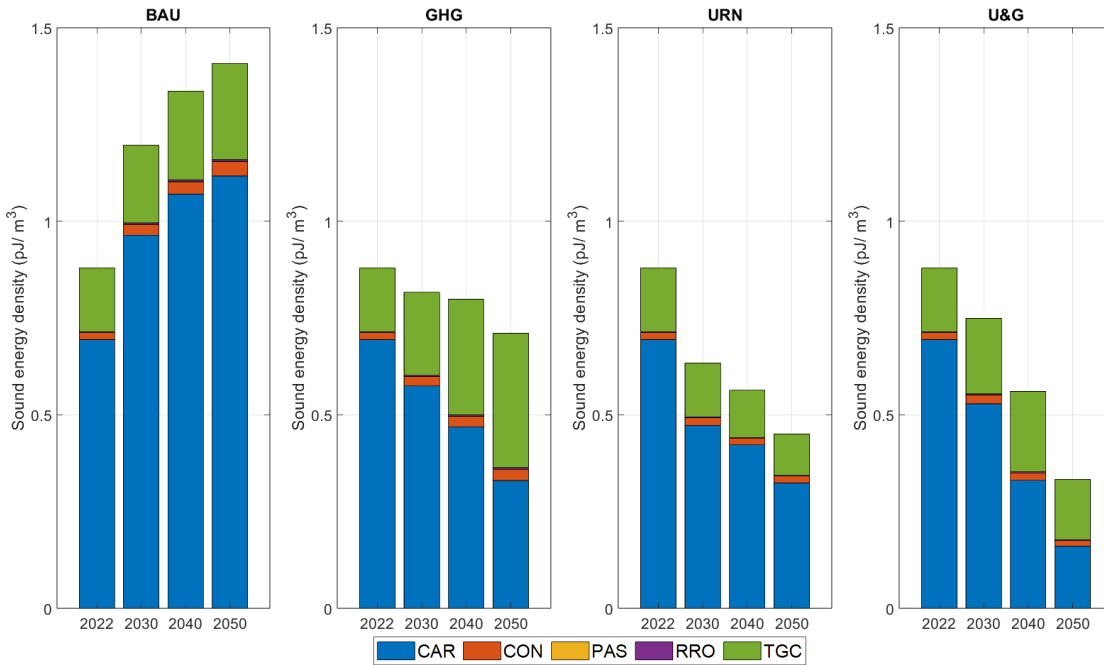
Figure 65 Black Sea: Forecast sound energy density categorised for the different years at 63 Hz.
