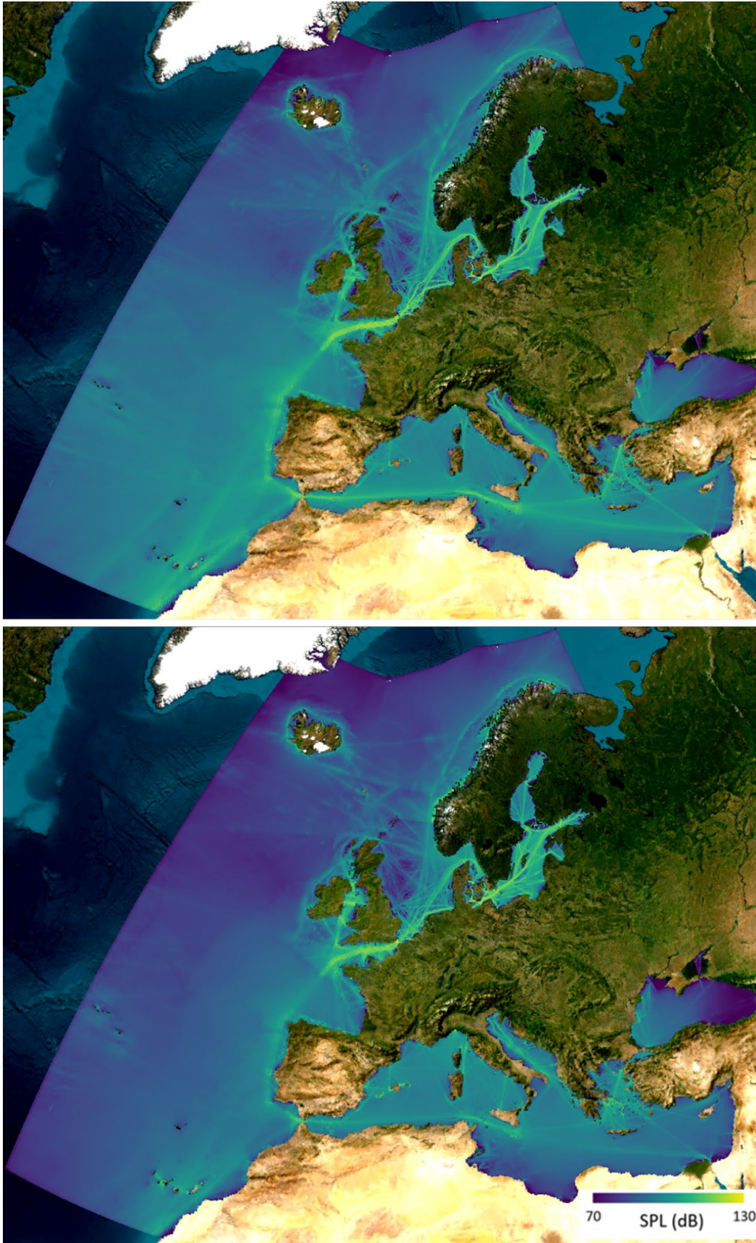
Figure 15 Europe: Sound map layers (SPL re 1 \mu\text{Pa}^2 , in dB) for 2022 including ALL vessel categories at (top) 63 Hz and (bottom) 125 Hz.
