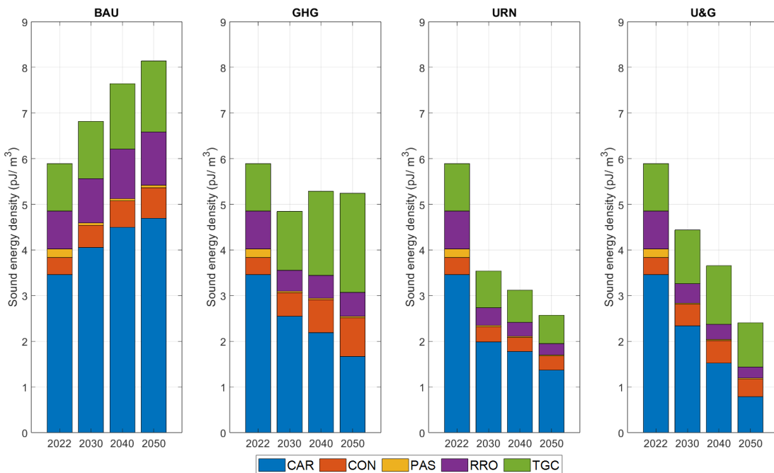
Figure 69 Mediterranean Sea: Forecast sound energy density categorised for the different years at 63 Hz.
