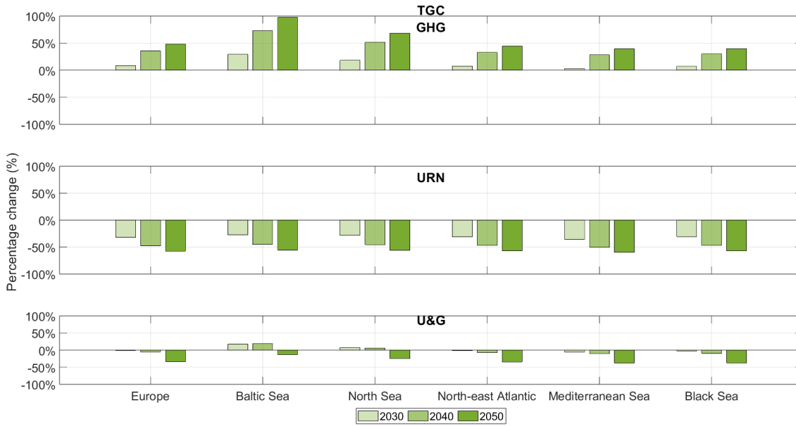
Figure 85 TGC vessel category: Comparing the percentage change in the forecast sound energy density at different regions at 63 Hz for GHG, (middle) URN, and (bottom) U&G forecast scenarios are shown in 2030, 2040, and 2050.
