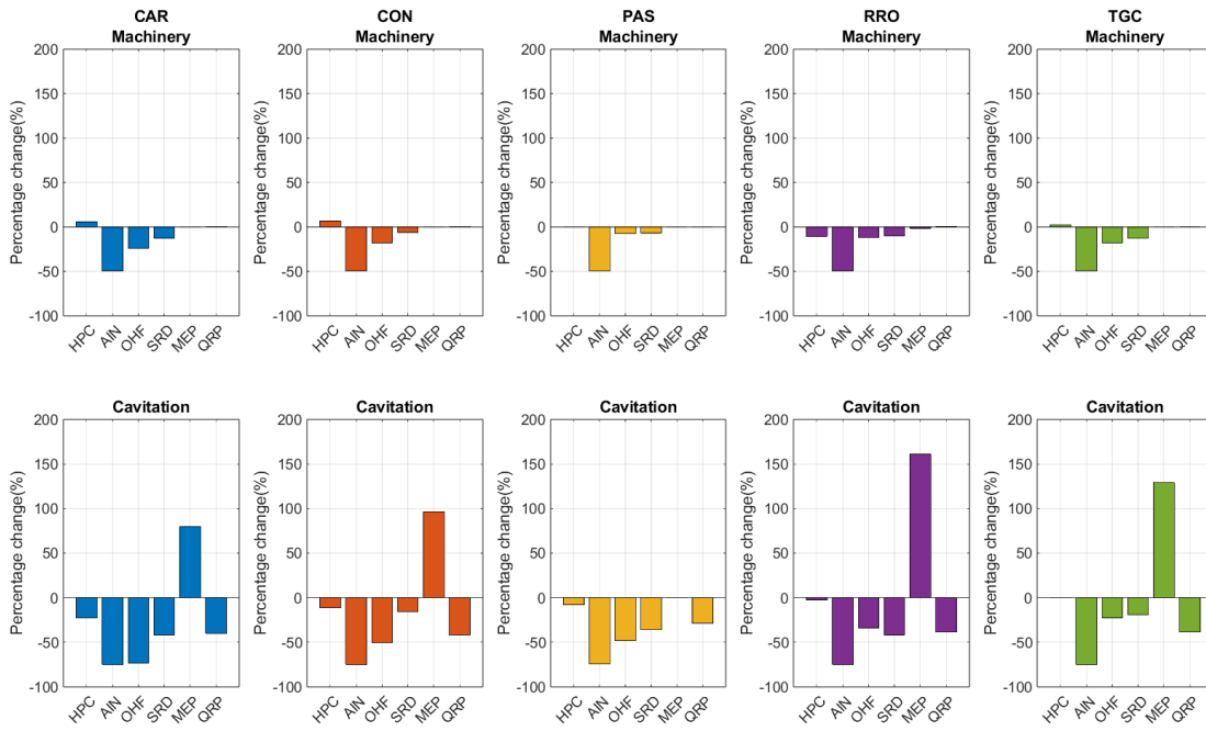
Figure 67 Black Sea: Forecast percentage change in the sound energy density for (top) machinery and (bottom) cavitation components compared to the BAU scenario at 63 Hz.
