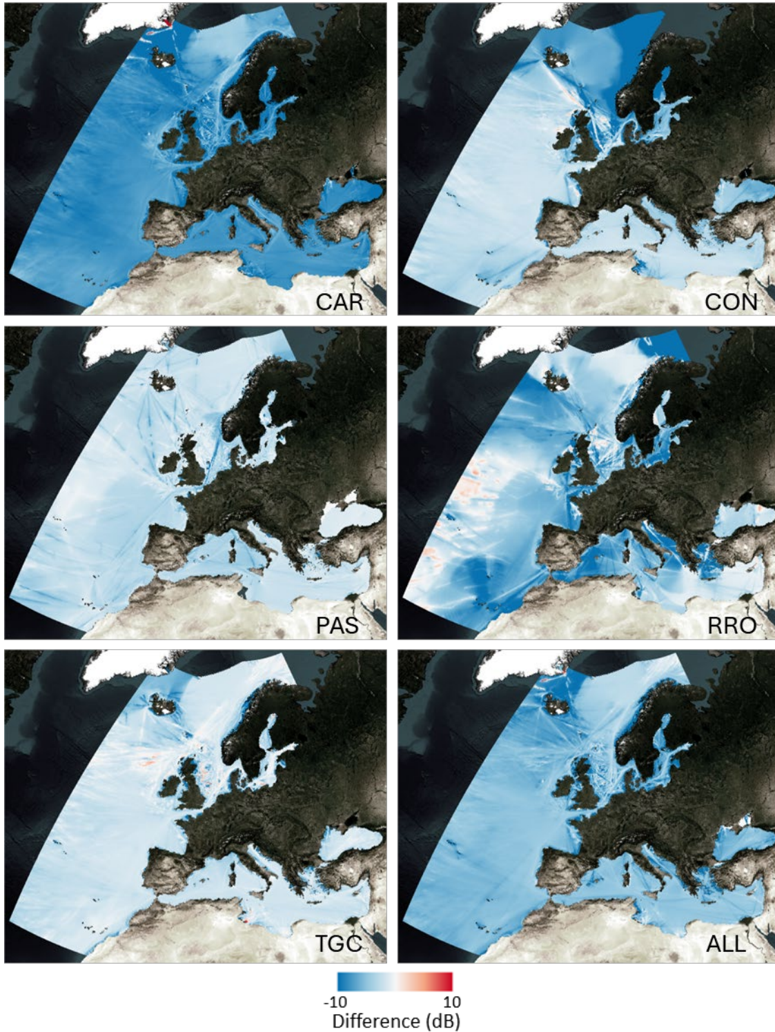
Figure 58 Difference in forecast sound pressure level (SPL; dB) for different vessel categories between BAU and U&G scenarios. The sound map layers are annually averaged for 2050 at 63 Hz.
