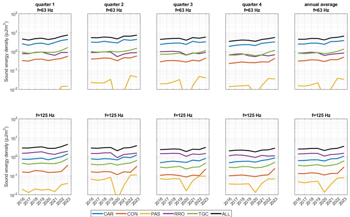
Figure 35 Mediterranean Sea: Sound energy density (in pJ/m³) of different vessel categories for each quarter and year for (top) 63 Hz and (bottom) 125 Hz.
