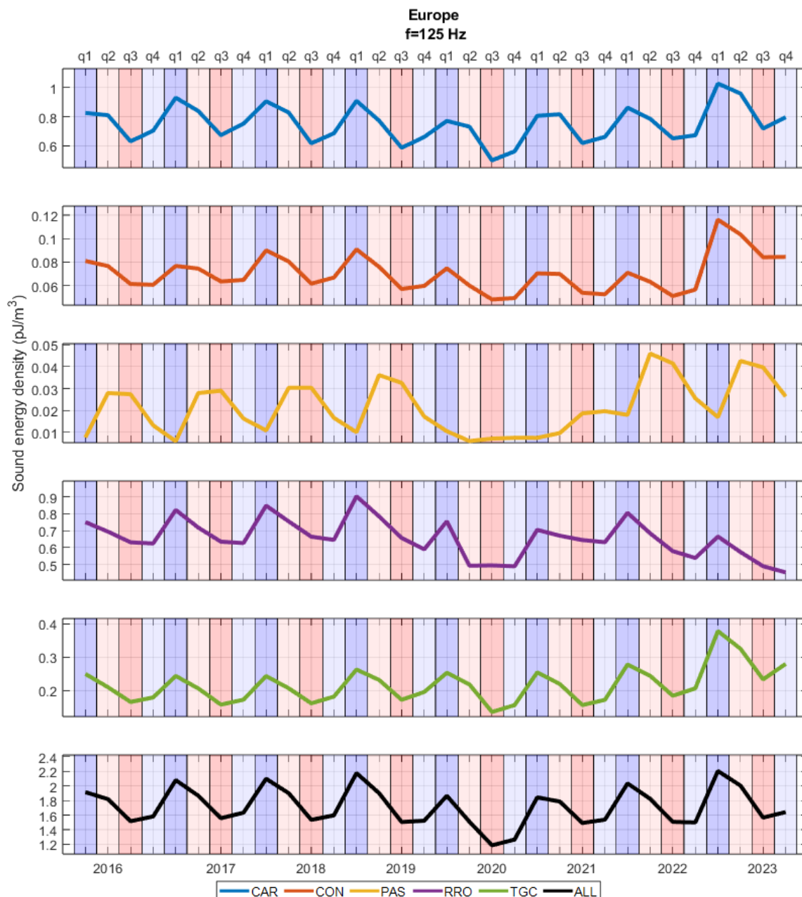
Figure 19 Europe: Sound energy density (in pJ/m 3 ) of different vessel categories for each quarter in chronological order at 125 Hz.
