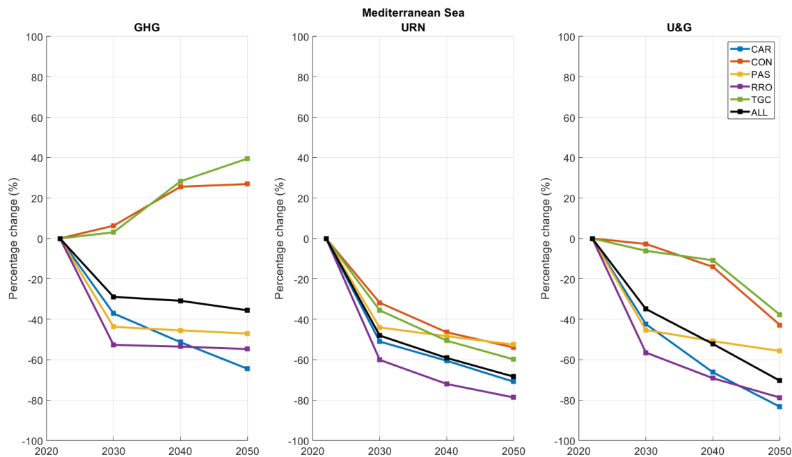
Figure 72 Mediterranean Sea: Forecast percentage change in the sound energy density compared to the BAU scenario at 63 Hz.
