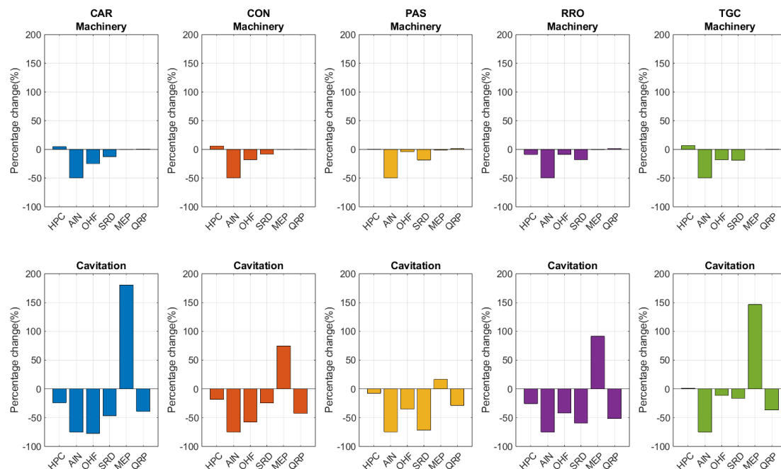
Figure 63 Baltic Sea: Forecast percentage change in the sound energy density for (top) machinery and (bottom) cavitation components compared to the BAU scenario at 63 Hz.
