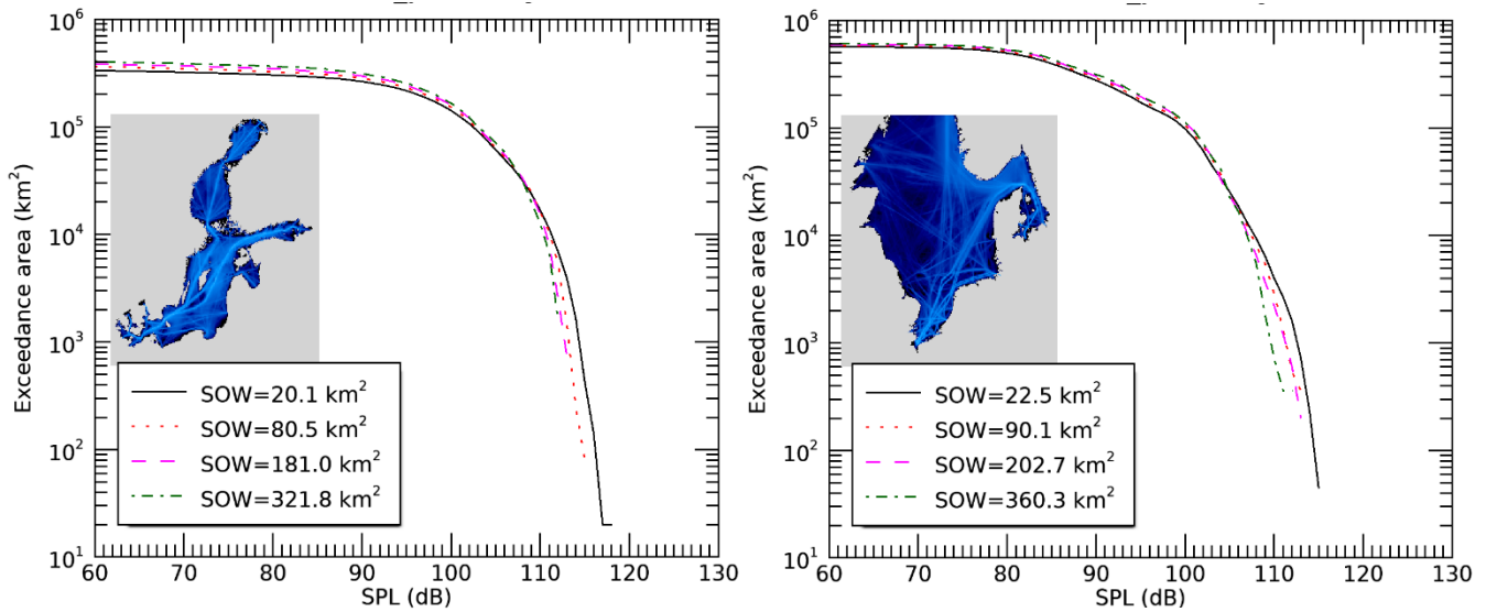
Figure 91 Exceedance area versus underwater noise limit value (UNLV) in the (left) Baltic Sea and (right) North Sea for different sizes of spatial observation window (SOW). Exceedance areas are calculated from the NAVISON 2022 yearly average sound maps. The exceedance area is plotted on a logarithmic scale.
