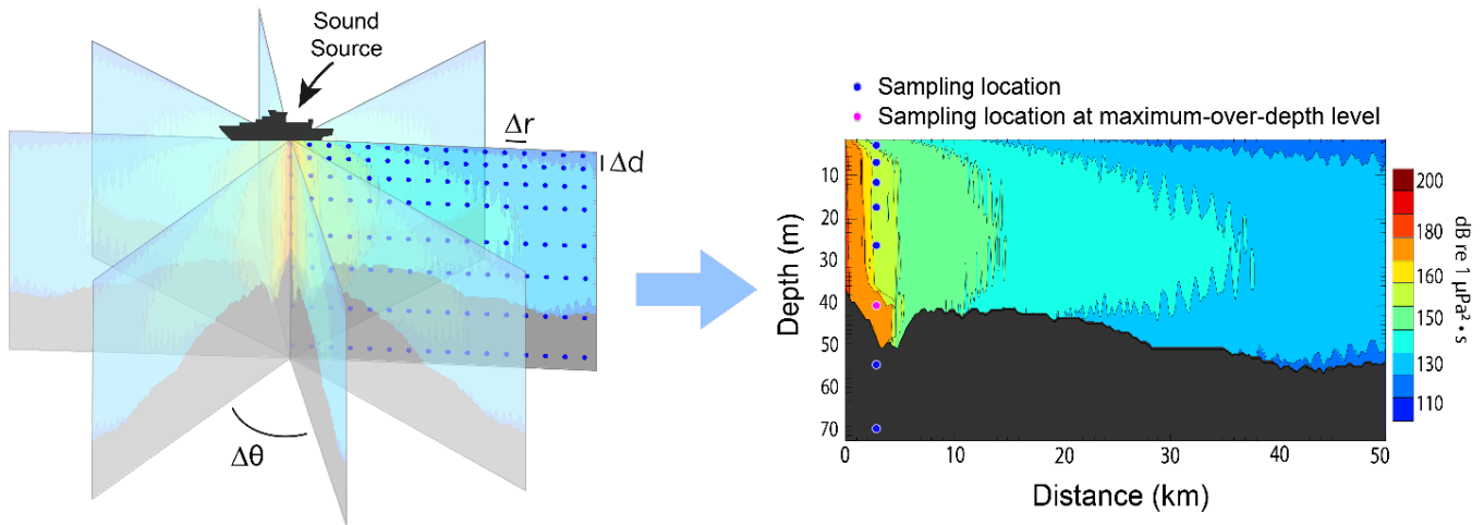
Figure 5 The N×2-D modelling in ARTEMIA, with each transect computed using CRAM.
