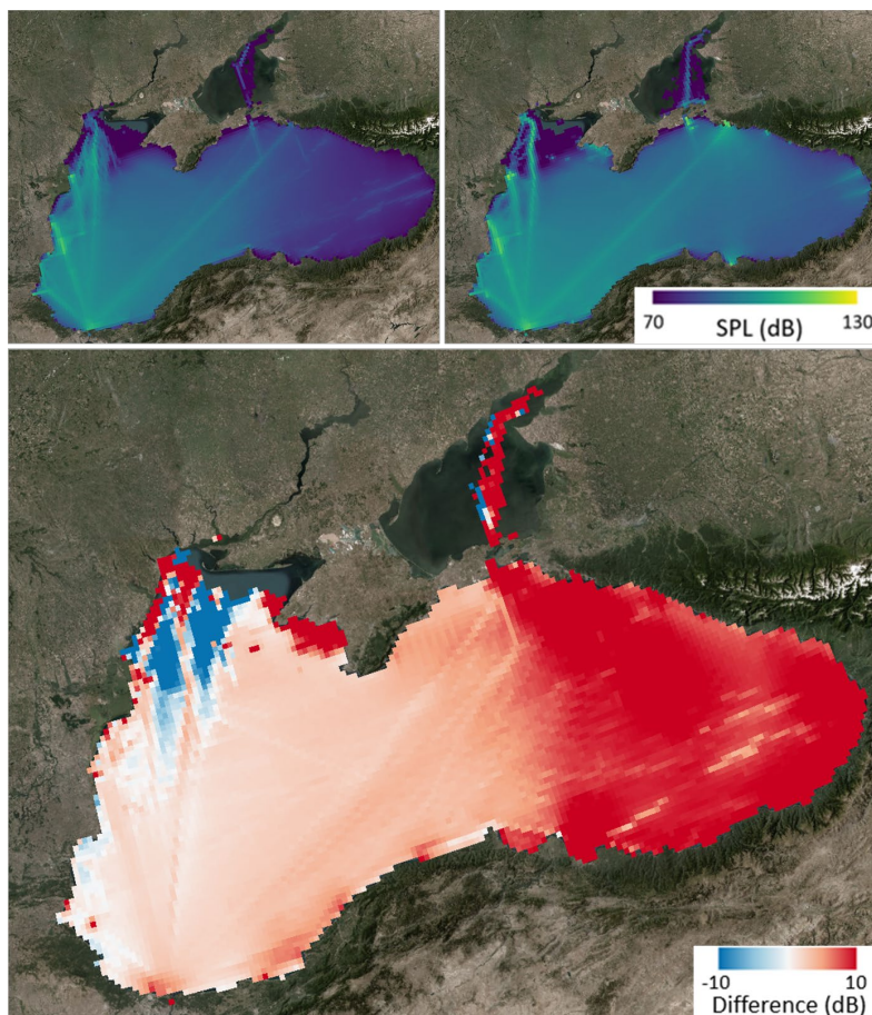
Figure 32 Black Sea: Sound map layers (SPL re 1 \mu\text{Pa}^2 , in dB) for (top left) 2022 and (top right) 2023 at 63 Hz. The (bottom) difference (2023–2022) of these two maps.
