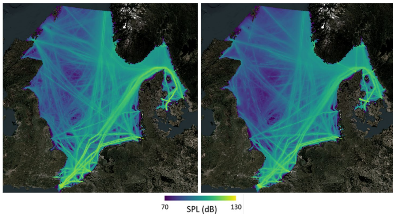
Figure 39 North Sea: Sound map layers (SPL re 1 \mu\text{Pa}^2 , in dB) for 2022 including ALL vessel categories at (left) 63 Hz and (right) 125 Hz.
