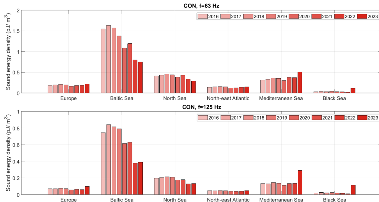
Figure 50 CON vessels: Sound energy density (in \text{pJ}/\text{m}^3 ) in different regions at (top) 63 Hz and (bottom) 125 Hz.
