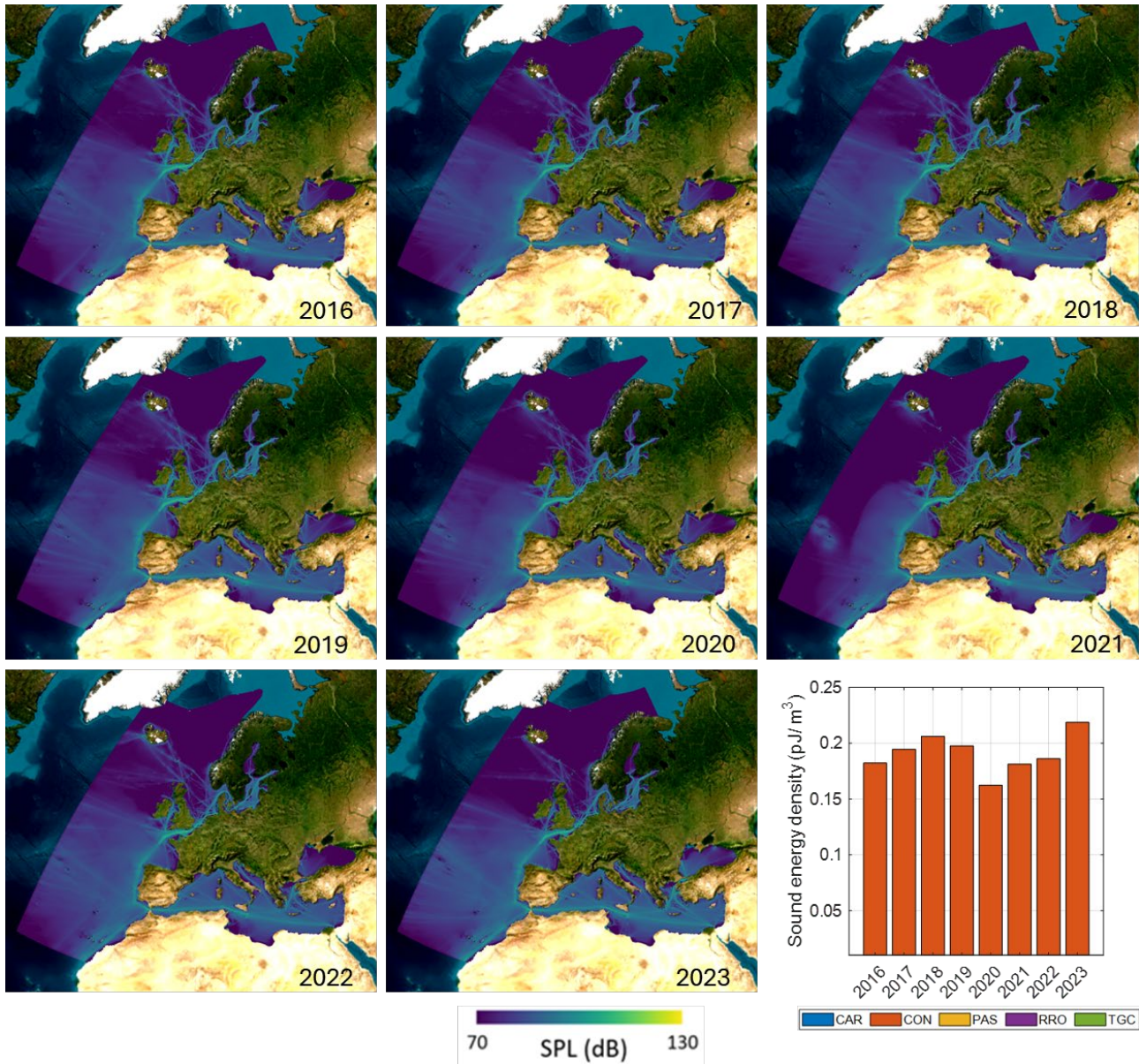
Figure 11 CON vessel categories: Annually averaged sound map layers (SPL re 1 \mu\text{Pa}^2 , in dB) including sound energy density (in \text{pJ}/\text{m}^3 ) at 63 Hz. One picojoule (1 pJ) is equal to one trillionth of a joule ( 10^{-12} J).
