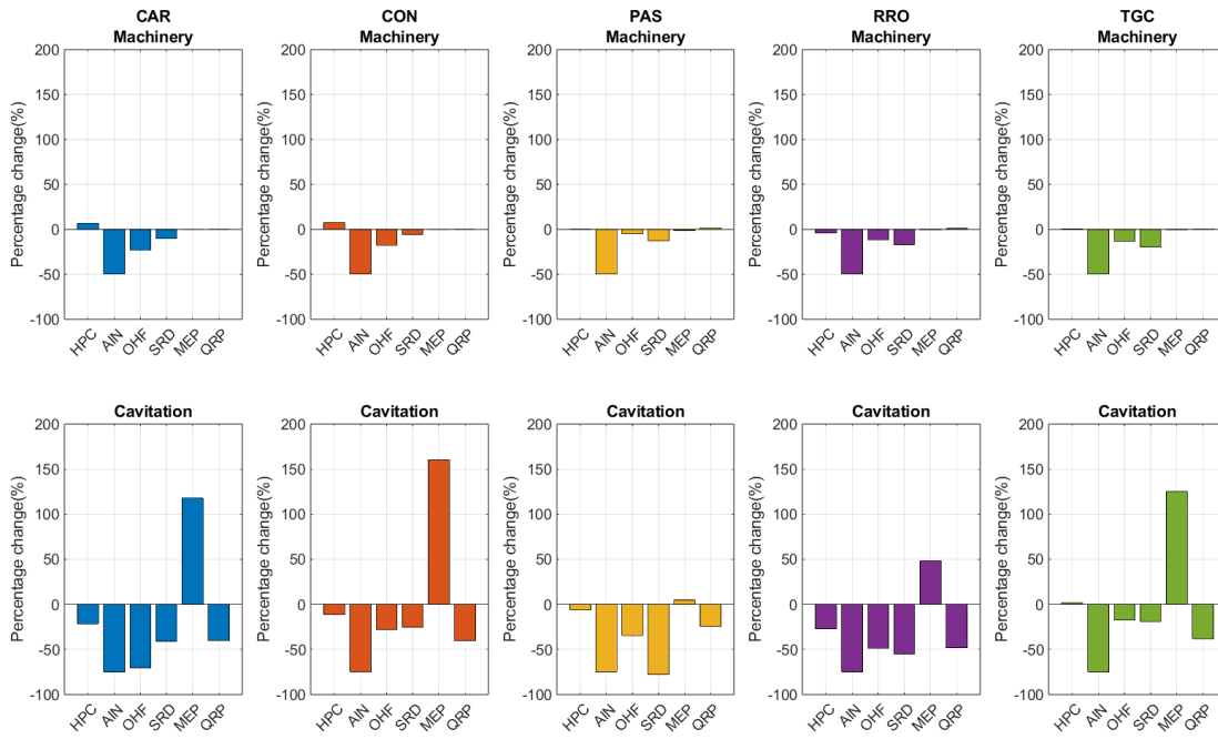
Figure 79 Northeast Atlantic Ocean: Forecast percentage change in the sound energy density for (top) machinery and (bottom) cavitation components compared to the BAU scenario at 63 Hz.
