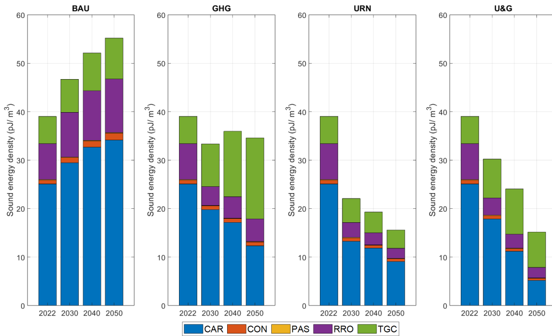
Figure 61 Baltic Sea: Forecast sound energy density categorised for the different years at 63 Hz.
