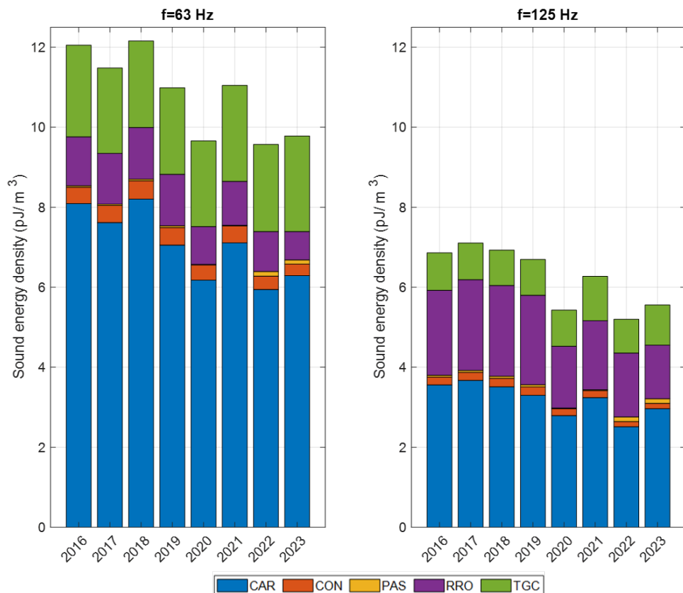
Figure 40 North Sea: Annually averaged sound energy density (in pJ/m³) at (left) 63 Hz and (right) 125 Hz.
