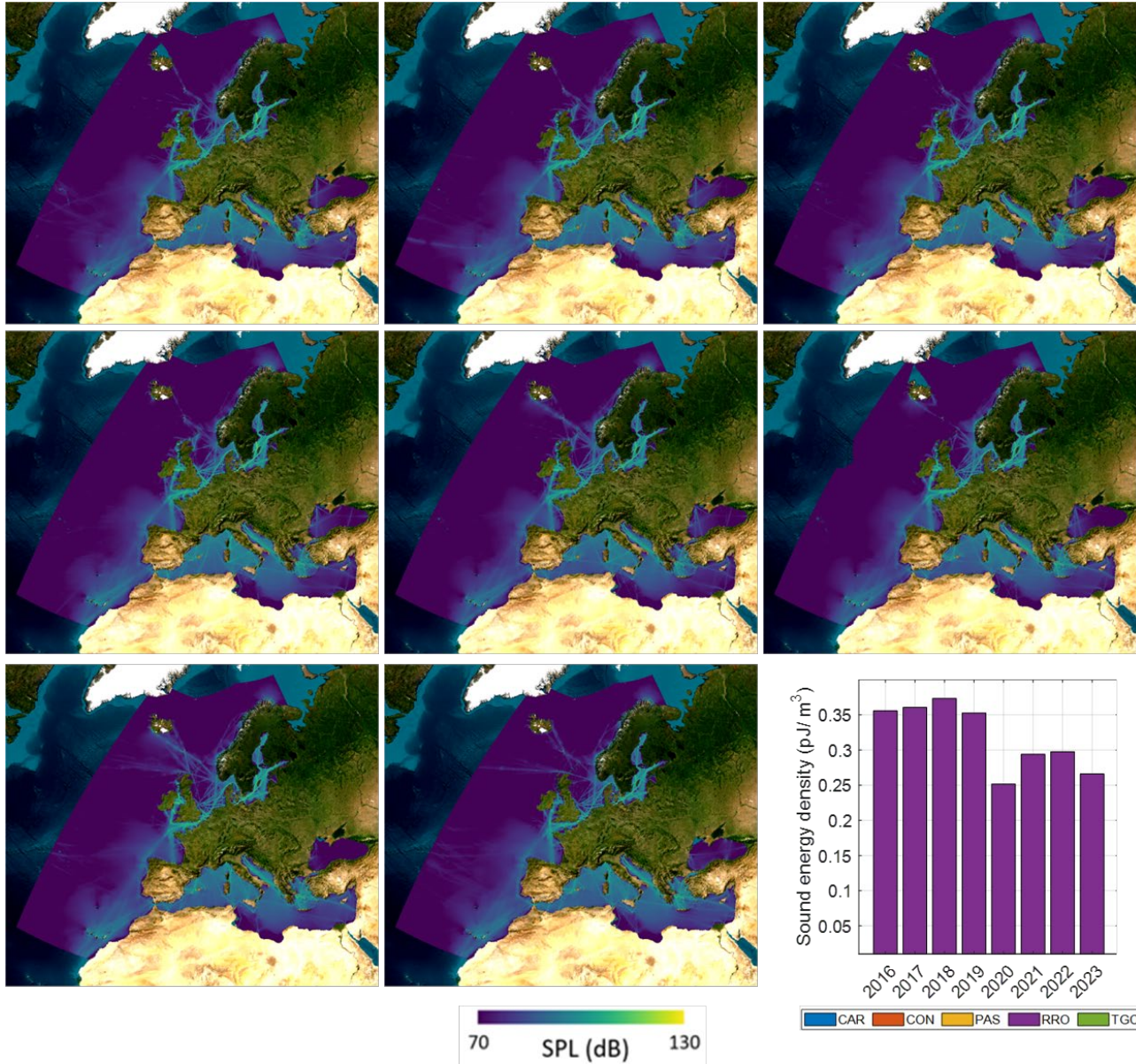
Figure 13 RRO vessel categories: Annually averaged sound map layers (SPL re 1 \mu\text{Pa}^2 , in dB) including sound energy density (in \text{pJ}/\text{m}^3 ) at 63 Hz. One picojoule (1 pJ) is equal to one trillionth of a joule ( 10^{-12} J).
