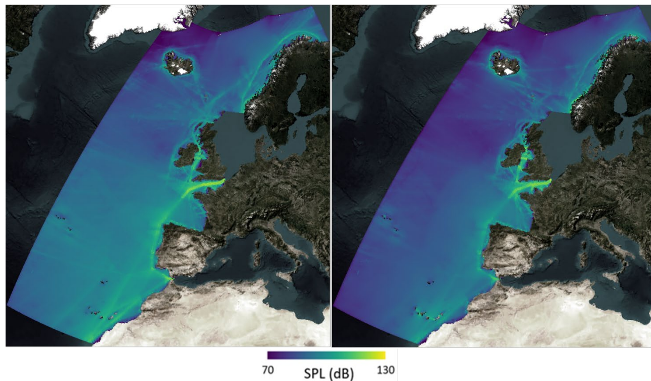
Figure 44 Northeast Atlantic Ocean: Sound map layers (SPL re 1 \mu\text{Pa}^2 , in dB) for 2022 including ALL vessel categories at (left) 63 Hz and (right) 125 Hz.
