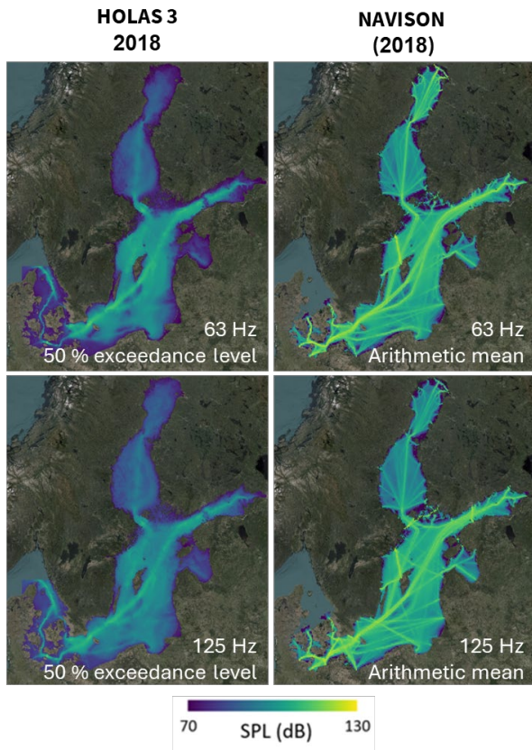
Figure 97 Comparison between (left) HOLAS 3 (HELCOM BLUES) and (right) NAVISON sound maps at (top) 63 Hz and (bottom) 125 Hz. The NAVISON results are based on spatially averaged sound pressure level while the HOLAS 3 (HELCOM BLUE) results are for the median (50th percentile) of SPL.
