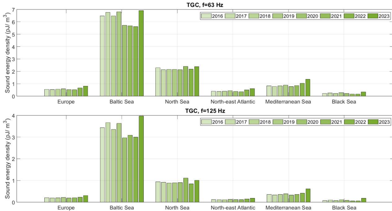
Figure 53 TGC vessels: Sound energy density (in pJ/m 3 ) in different regions at (top) 63 Hz and (bottom) 125 Hz.
