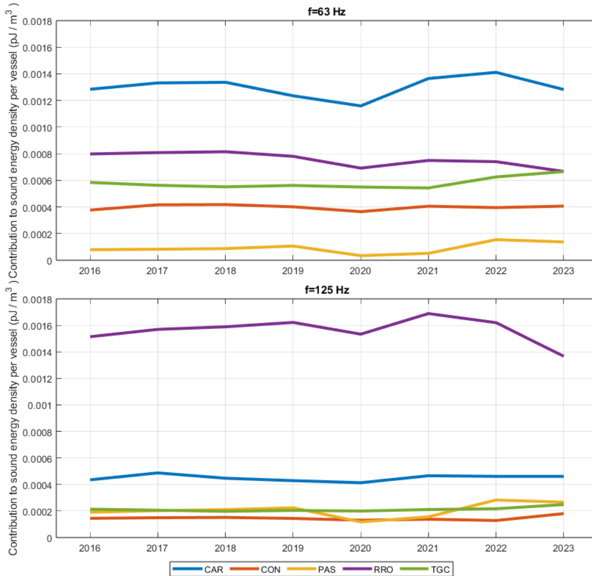
Figure 21 Europe: Annual variation of average contribution to sound energy density (in pJ/m³) per vessel for each vessel category for (top) 63 Hz and (bottom) 125 Hz.
