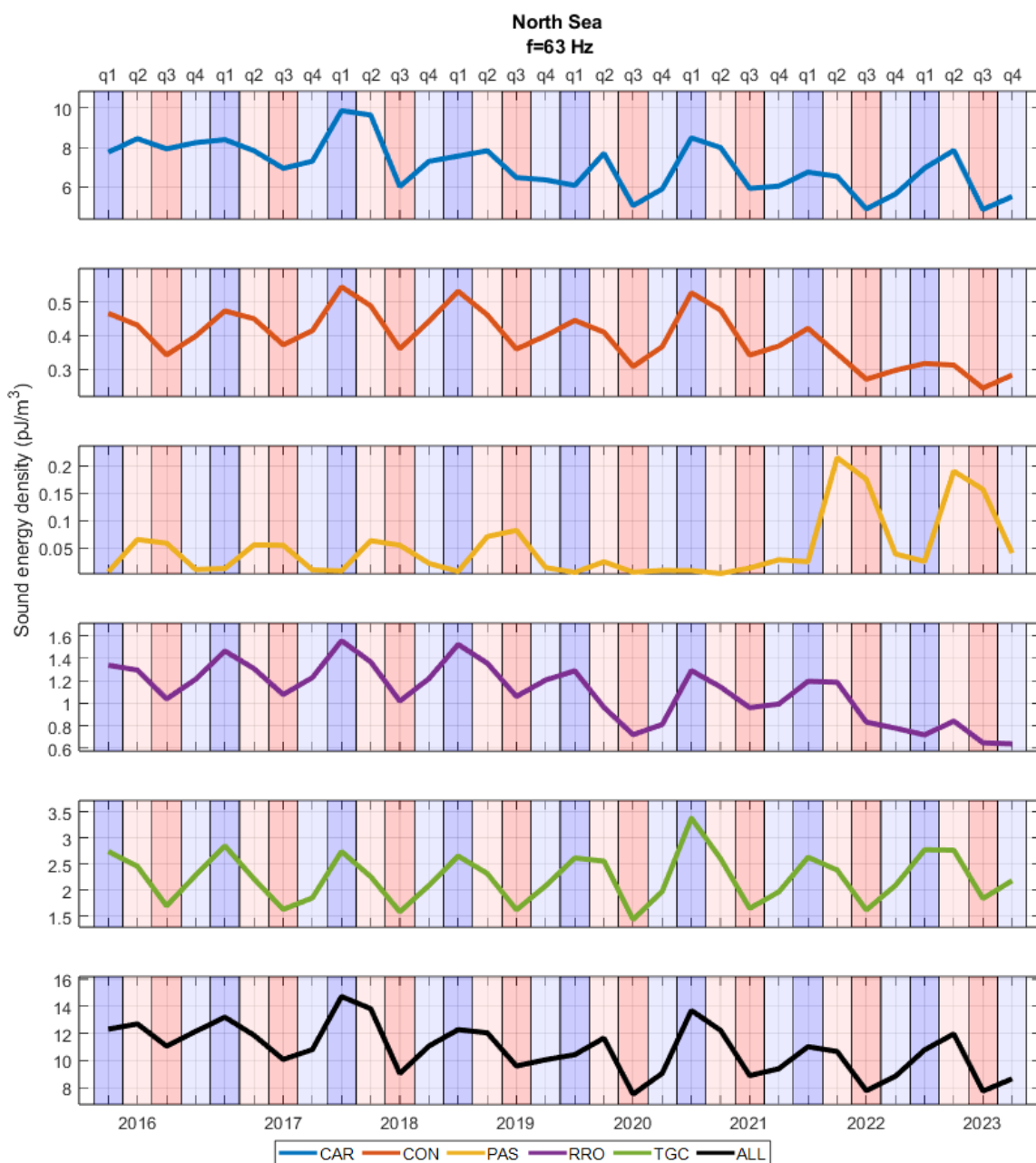
Figure 42 North Sea: Sound energy density (in pJ/m 3 ) of different vessel categories for each quarter in chronological order at 63 Hz.
