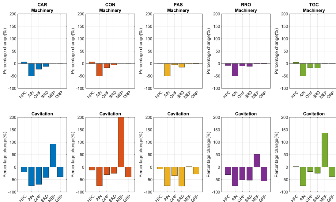
Figure 71 Mediterranean Sea: Forecast percentage change in the sound energy density for (top) machinery and (bottom) cavitation components compared to the BAU scenario at 63 Hz.
