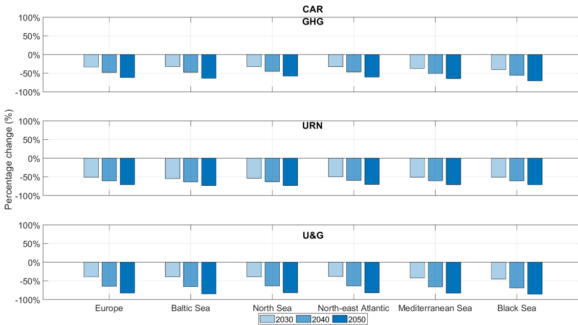
Figure 81 CAR vessel category: Comparing the percentage change in the forecast sound energy density at different regions at 63 Hz for GHG (top), URN (middle), and U&G (bottom) forecast scenarios are shown in 2030, 2040, and 2050.
