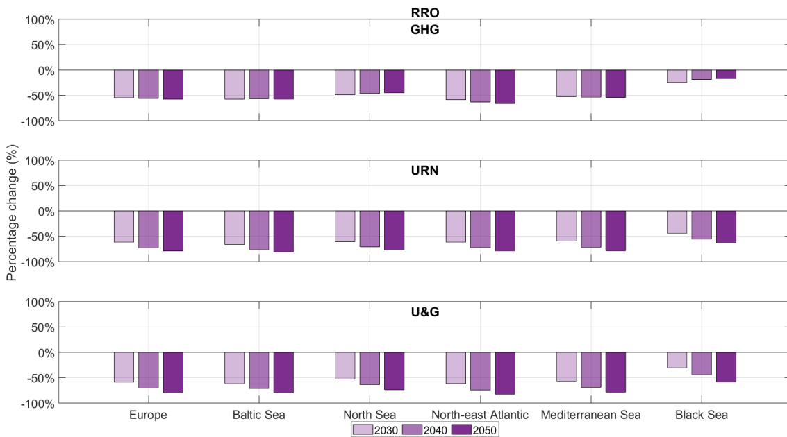
Figure 84 RRO vessel category: Comparing the percentage change in the forecast sound energy density at different regions at 63 Hz for GHG, (middle) URN, and (bottom) U&G forecast scenarios are shown in 2030, 2040, and 2050.
