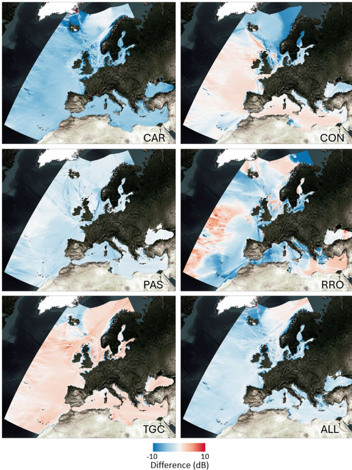
Figure 56 Difference in forecast sound pressure level (SPL; dB) for different vessel categories between BAU and GHG scenarios. The sound map layers are annually averaged for 2050 at 63 Hz.
