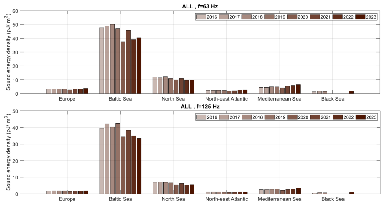
Figure 54 ALL vessels: Sound energy density (in pJ/m 3 ) in different regions at (top) 63 Hz and (bottom) 125 Hz.
