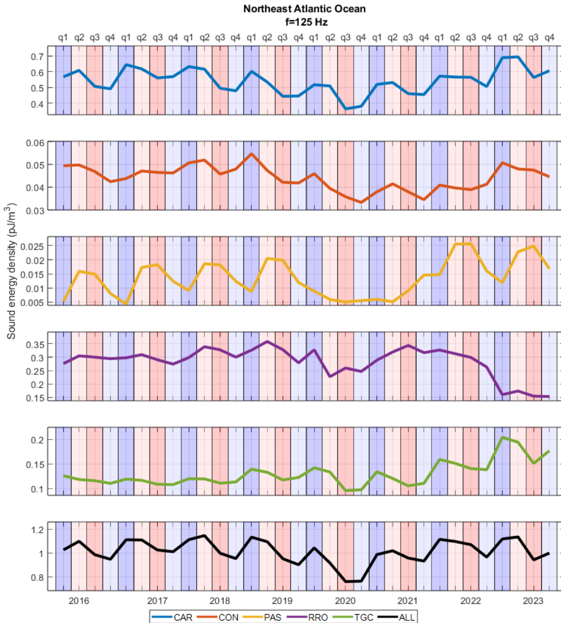
Figure 48 Northeast Atlantic Ocean: Sound energy density (in pJ/m 3 ) of different vessel categories for each quarter in chronological order at 125 Hz.
