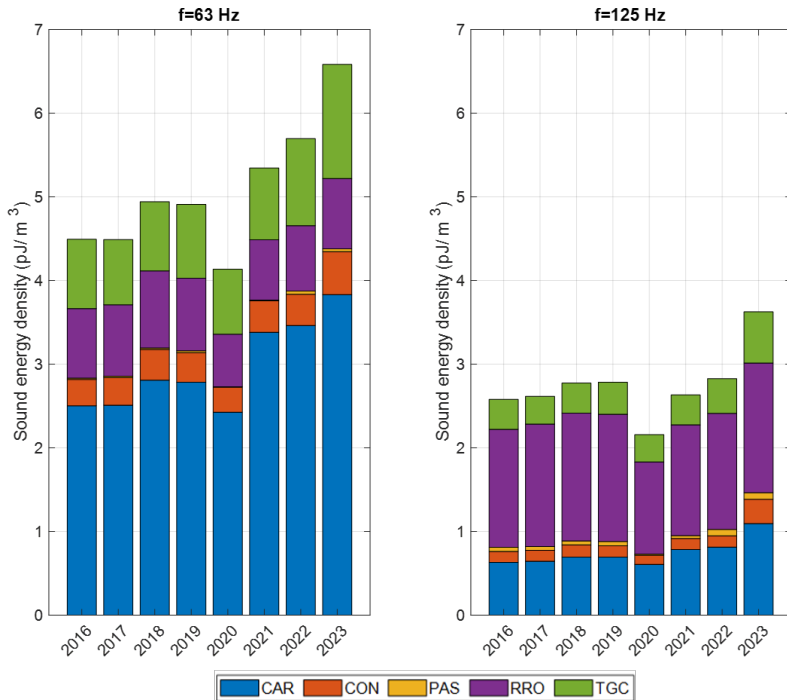
Figure 34 Mediterranean Sea: Annually averaged sound energy density (in pJ/m³) at (left) 63 Hz and (right) 125 Hz.
