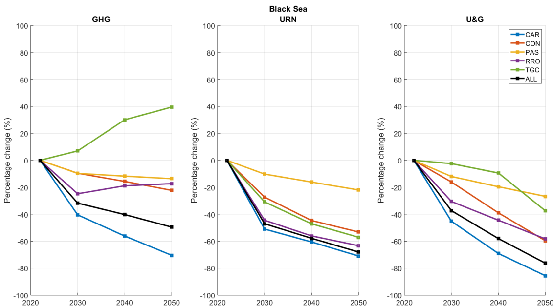
Figure 68 Black Sea: Forecast percentage change in the sound energy density compared to the BAU scenario at 63 Hz.
