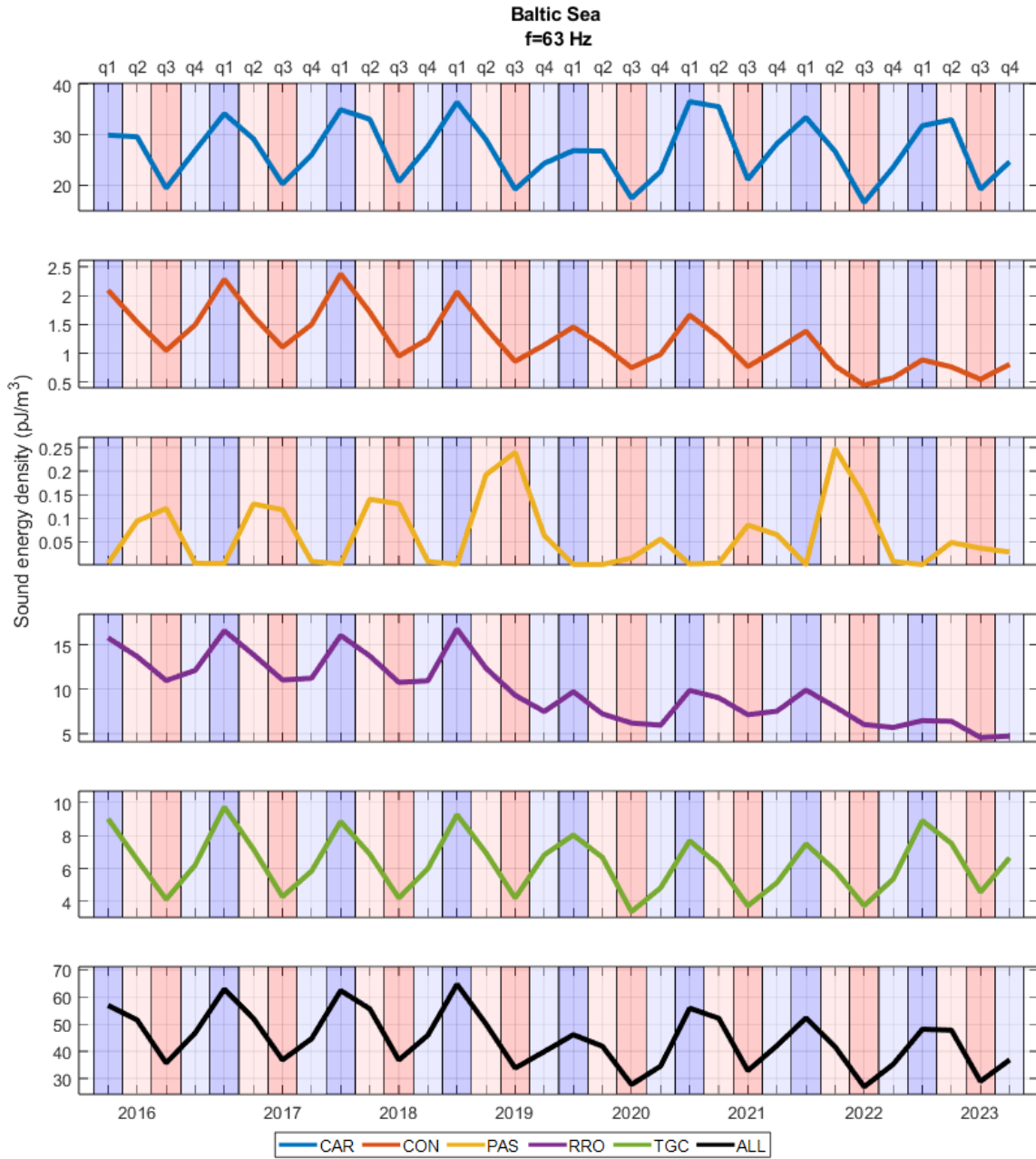
Figure 25 Baltic Sea: Sound energy density (in pJ/m 3 ) of different vessel categories for each quarter in chronological order at 63 Hz.
