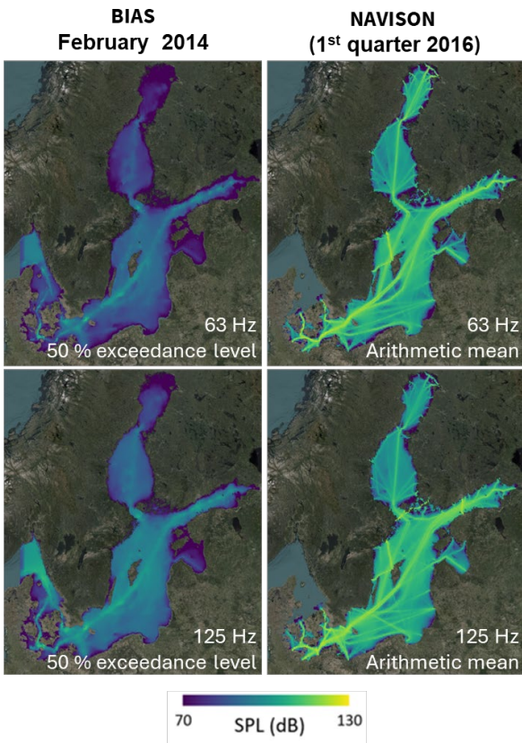
Figure 93 Comparison between (left) BIAS and (right) NAVISON sound maps (SPL re 1 \mu\text{Pa}^2 , in dB) at (top) 63 Hz and (bottom) 125 Hz. The NAVISON results are based on the spatially averaged sound pressure level while the BIAS results are for the median (spatio-temporal 50 % exceedance level). See Table 8 for detailed description of the metrics for each project.
