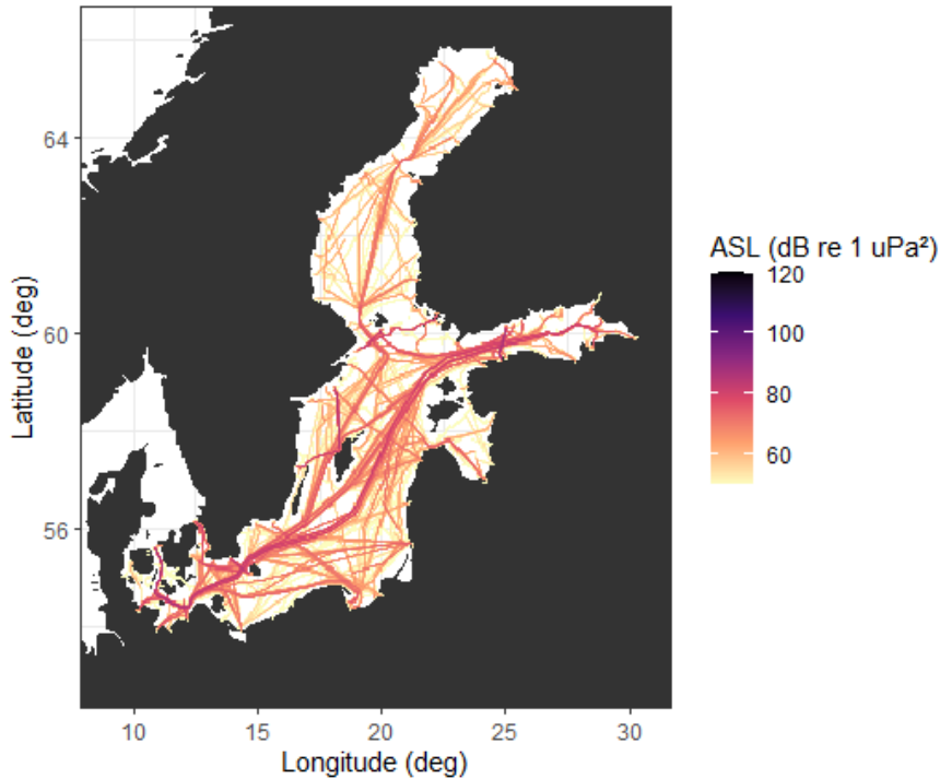
Figure 4 Example grid of areic source level (ASL) for the Baltic Sea in the 63 Hz decidecade band.
