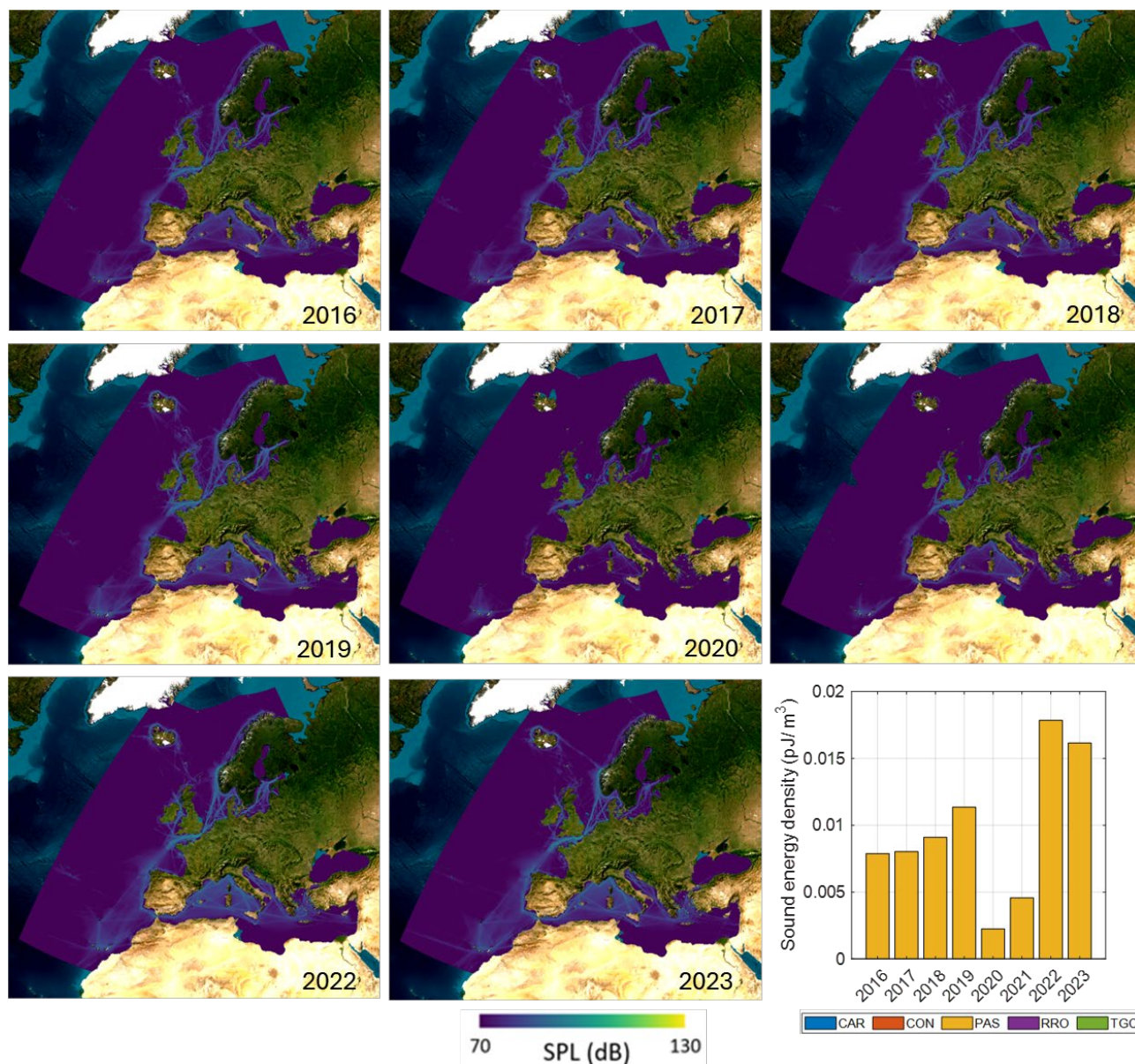
Figure 12 PAS vessel categories: Annually averaged sound map layers (SPL re \mu\text{Pa}^2 , in dB) including sound energy density (in \text{pJ}/\text{m}^3 ) at 63 Hz. One picojoule (1 pJ) is equal to one trillionth of a joule ( 10^{-12} J).
