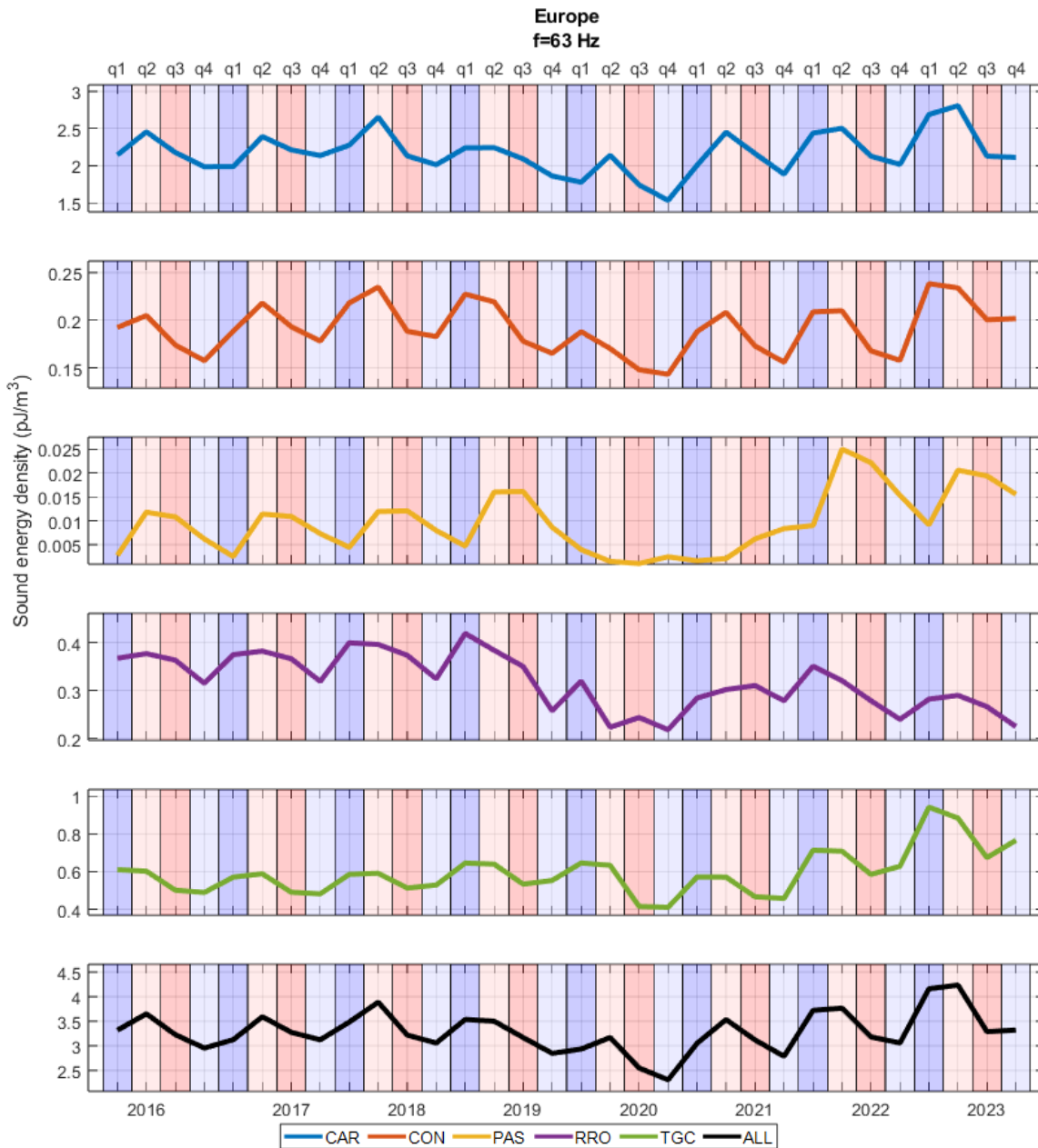
Figure 18 Europe: Sound energy density (in pJ/m 3 ) of different vessel categories for each quarter in chronological order at 63 Hz.
