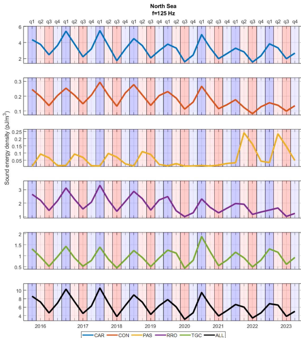
Figure 43 North Sea: Sound energy density (in pJ/m 3 ) of different vessel categories for each quarter in chronological order at 125 Hz.
