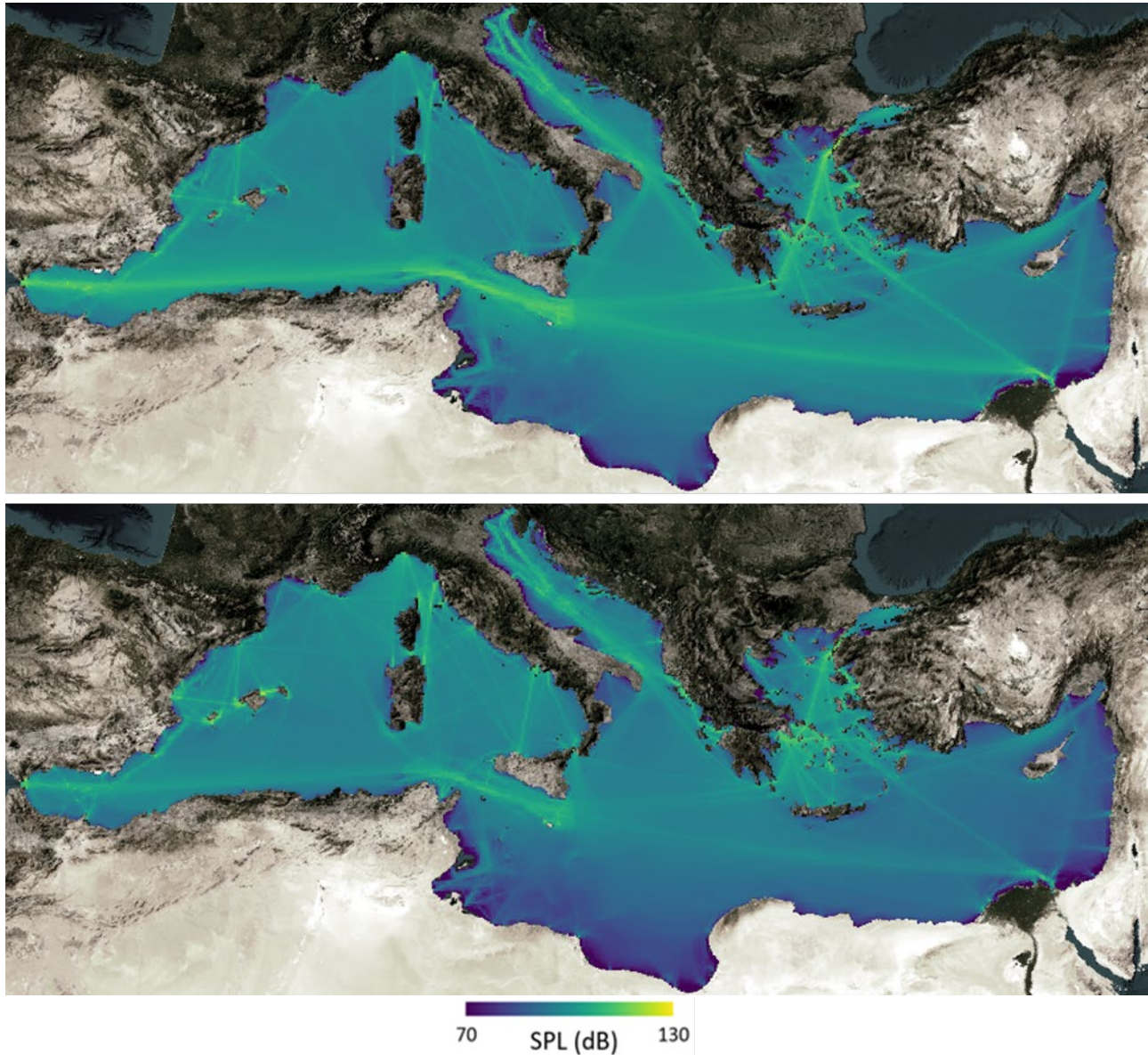
Figure 33 Mediterranean Sea: Sound map layers (SPL re 1 \mu\text{Pa}^2 , in dB) for 2022 including ALL vessel categories at (top) 63 Hz and (bottom) 125 Hz.
