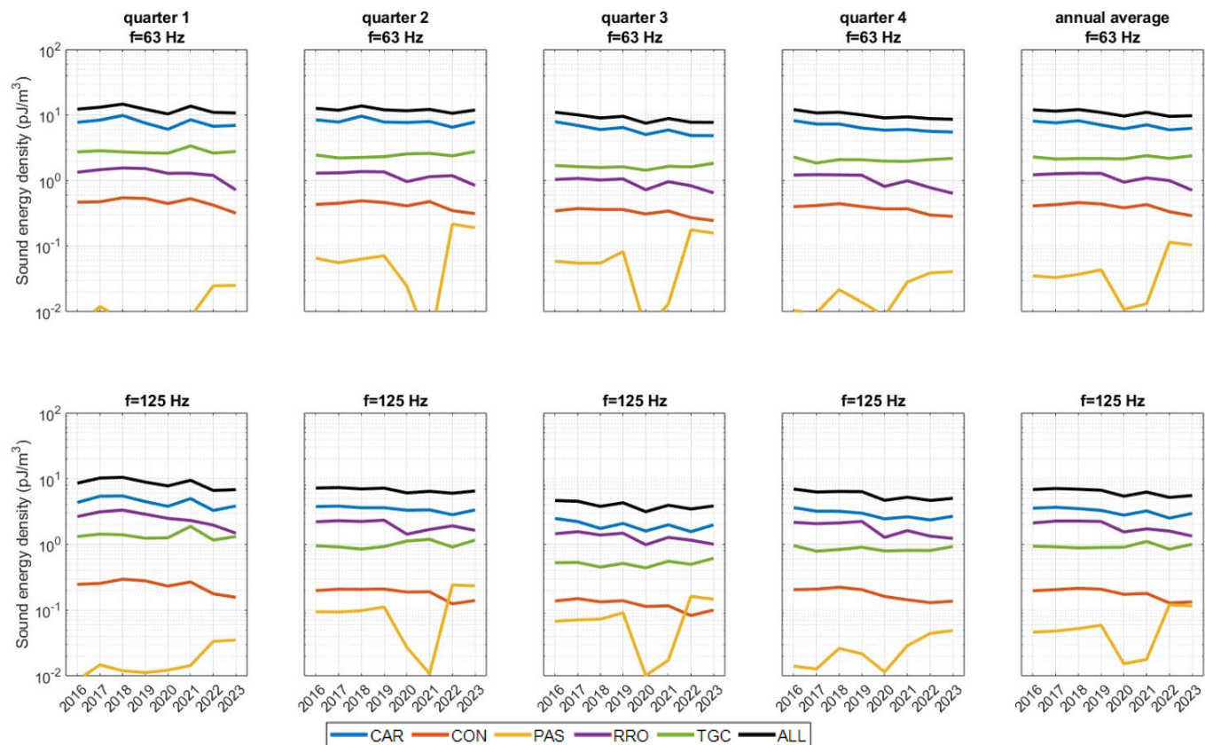
Figure 41 North Sea: Sound energy density (in pJ/m³) of different vessel categories for each quarter and year for (top) 63 Hz and (bottom) 125 Hz.
