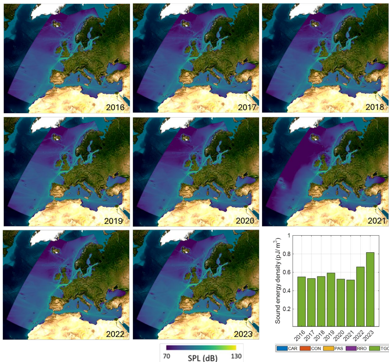
Figure 14 TGC vessel categories: Annually averaged sound map layers (SPL re 1 \mu\text{Pa}^2 , in dB) including sound energy density (in \text{pJ}/\text{m}^3 ) at 63 Hz. One picojoule (1 pJ) is equal to one trillionth of a joule ( 10^{-12} J).
