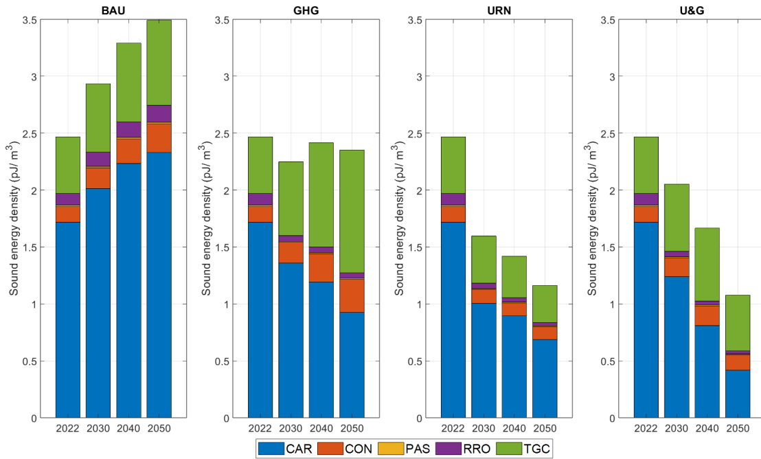
Figure 77 Northeast Atlantic Ocean: Forecast sound energy density categorised for the different years at 63 Hz.
