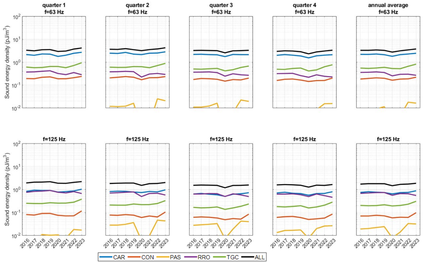
Figure 17 Europe: Sound energy density (in pJ/m³) for 2016 to 2023 of different vessel categories for each quarter and year for (top) 63 Hz and (bottom) 125 Hz.
