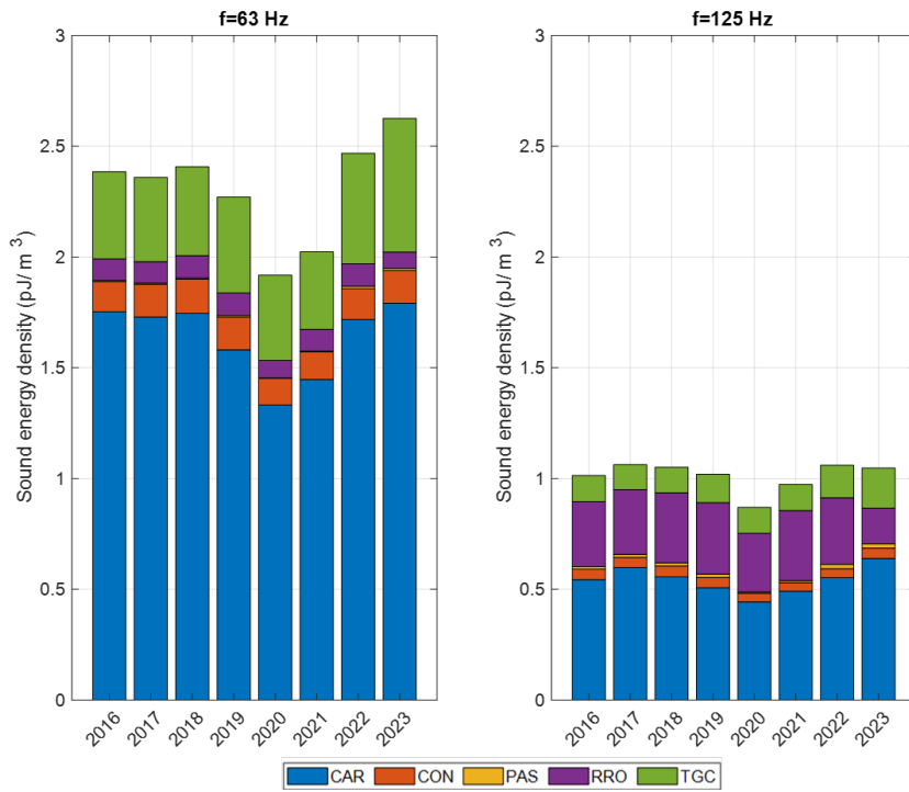
Figure 45 Northeast Atlantic Ocean: Annually averaged sound energy density (in pJ/m 3 ) at (left) 63 Hz and (right) 125 Hz.
