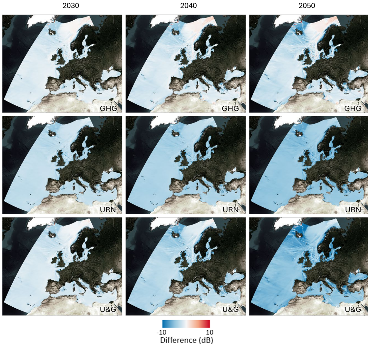
Figure 55 Difference in forecast sound pressure level (SPL; dB) including all vessel categories between BAU and (top) GHG, (middle) URN, and (bottom) U&G scenarios. These maps are produced for (left) 2030, (middle) 2040, and (right) 2050 at 63 Hz.
