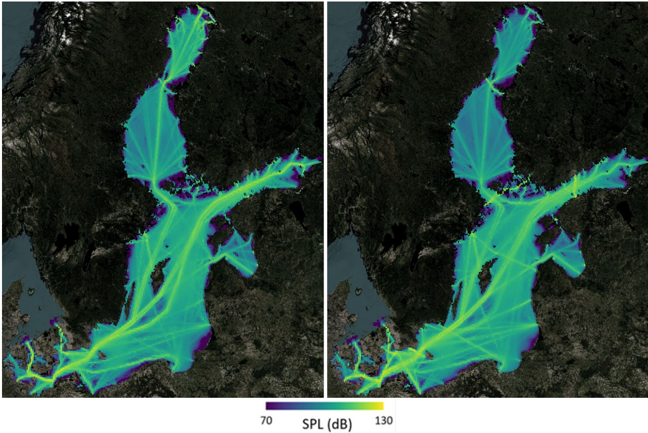
Figure 22 Baltic Sea: Sound map layers (SPL re 1 \mu\text{Pa}^2 , in dB) for 2022 including ALL vessel categories at (left) 63 Hz and (right) 125 Hz.
