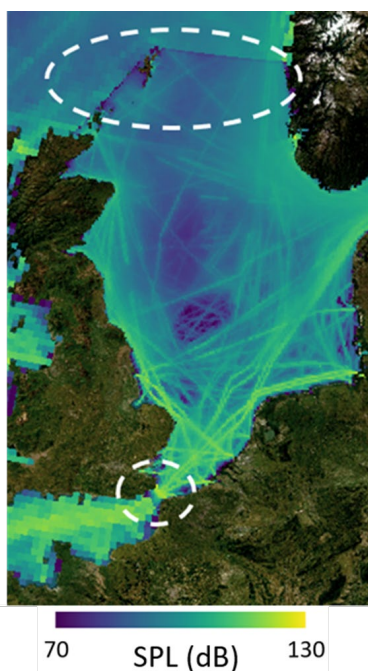
Figure 88 Artefacts at the North Sea boundaries (Sound pressure level re 1 \mu\text{Pa}^2 (dB)). The artefacts that appear as straight blue lines (highlighted in the white circles) for the visualisation of individual hindcast sound pressure level map layers in QGIS.
