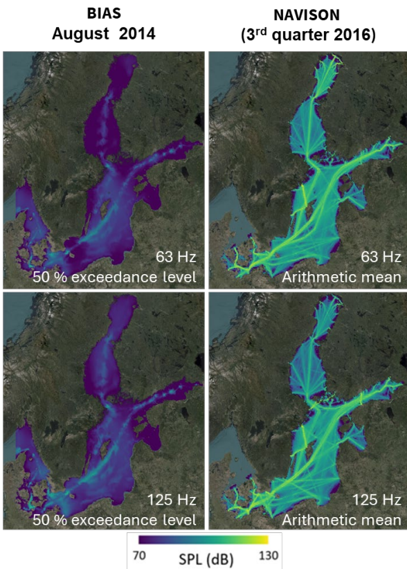
Figure 94 Comparison between (left) BIAS and (right) NAVISON sound maps (SPL re 1 \mu\text{Pa}^2 , in dB) at (top) 63 Hz and (bottom) 125 Hz. The NAVISON results are based on spatially averaged sound pressure level while the BIAS results are for the median (spatio-temporal 50 % exceedance level). See Table 8 for detailed description of the metrics for each project.
