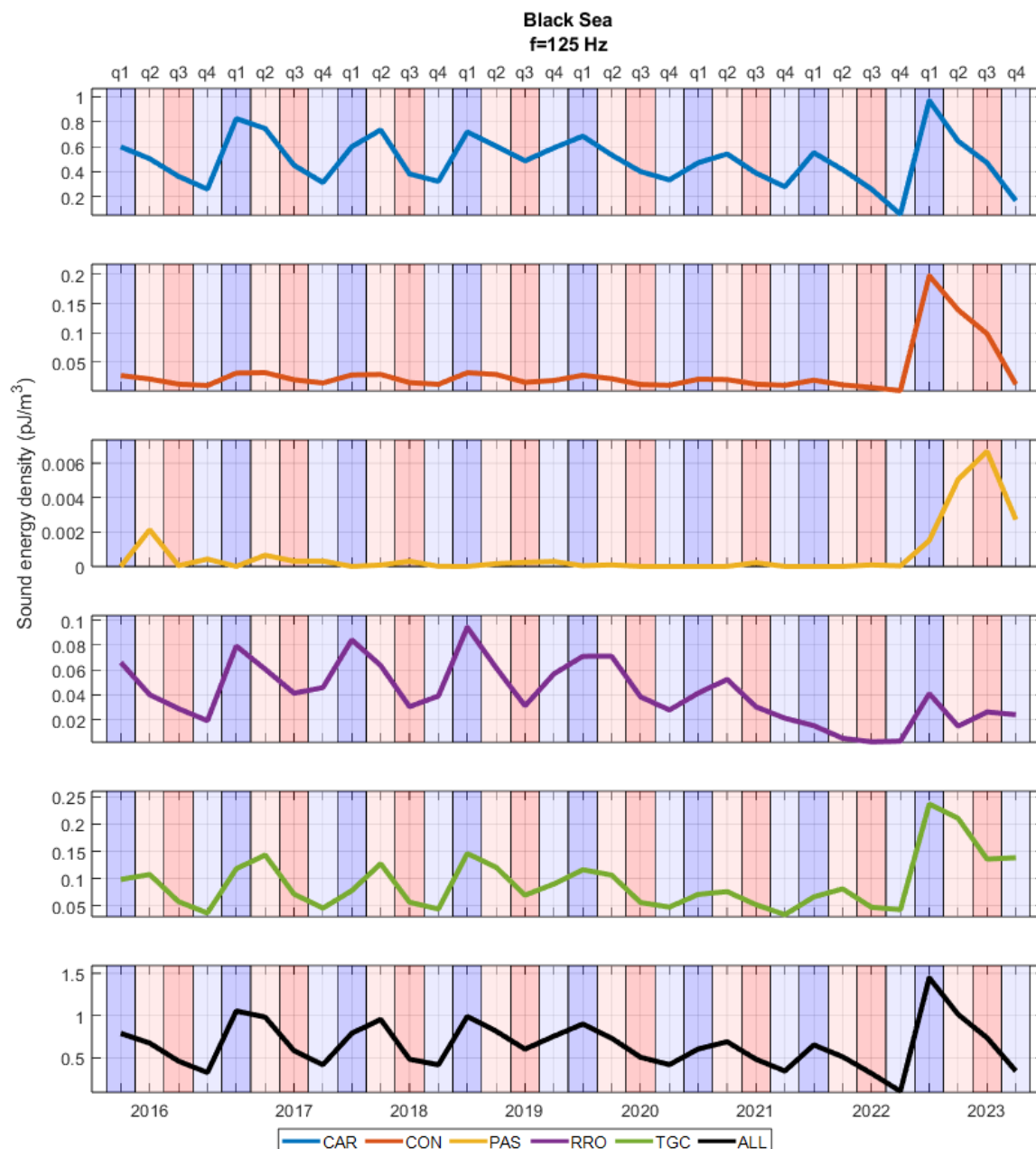
Figure 31 Black Sea: Sound energy density (in pJ/m 3 ) of different vessel categories for each quarter in chronological order at 125 Hz.
