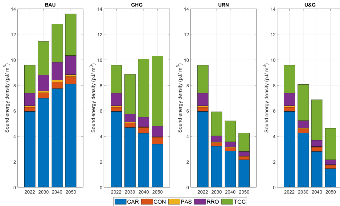
Figure 73 North Sea: Forecast sound energy density categorised for the different years at 63 Hz.
