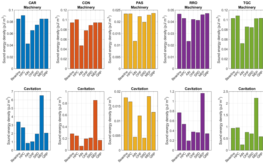
Figure 70 Mediterranean Sea: Forecast sound energy density for the 100 % penetration rates for each mitigation measure at 63 Hz. Sound energy density is calculated for (top) machinery and (bottom) cavitation components.
