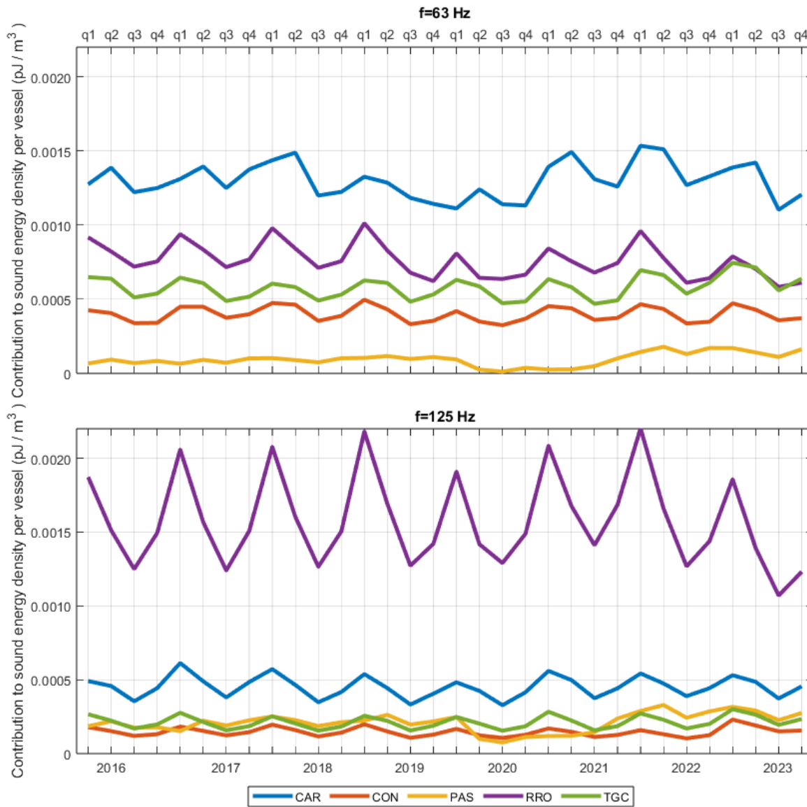
Figure 20 Europe: Quarterly variation of average contribution to sound energy density (in pJ/m 3 ) per vessel for each vessel category for (top) 63 Hz and (bottom) 125 Hz.
