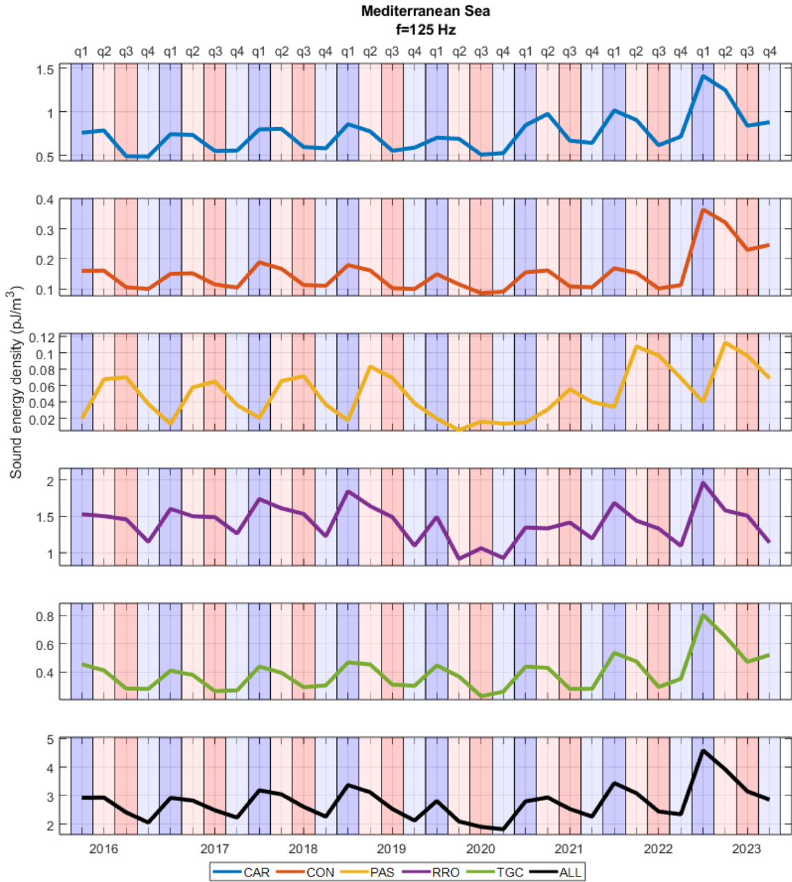
Figure 38 Mediterranean Sea: Sound energy density (in \text{pJ/m}^3 ) of different vessel categories for each quarter in chronological order for 125 Hz.
