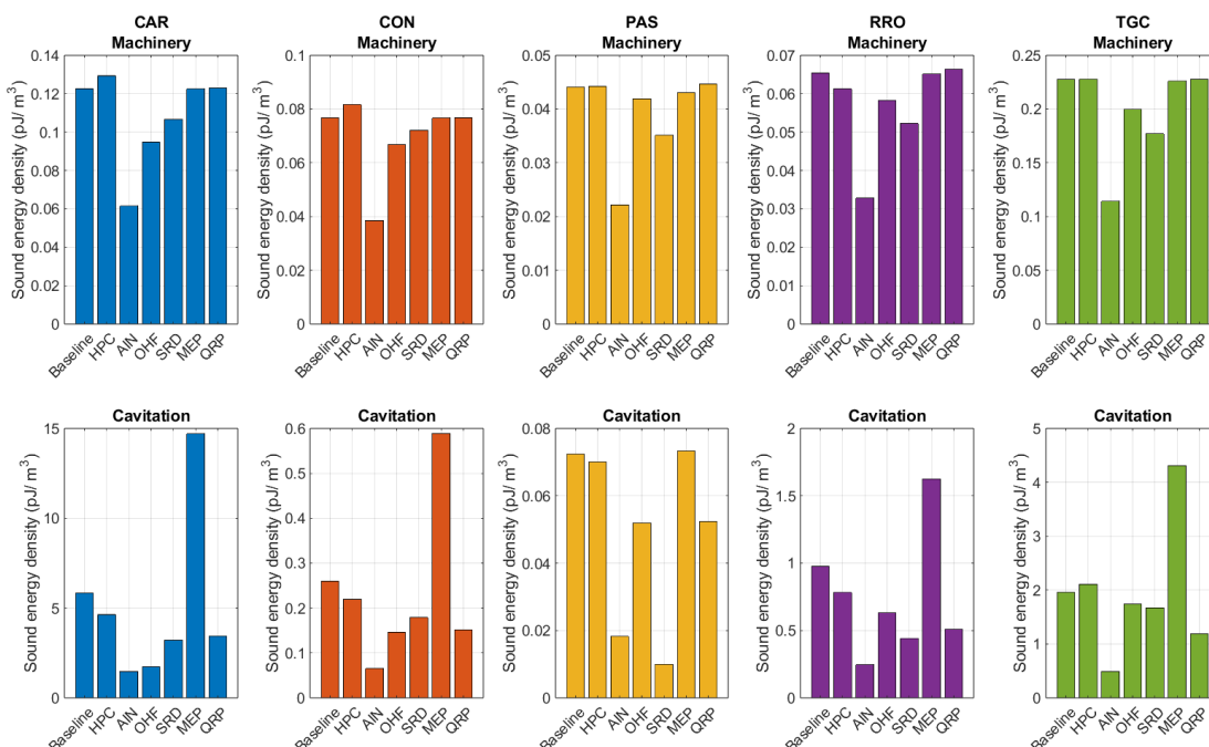
Figure 74 North Sea: Forecast sound energy density for the 100 % penetration rates for each mitigation measure at 63 Hz. Sound energy density is calculated for (top) machinery and (bottom) cavitation components.
