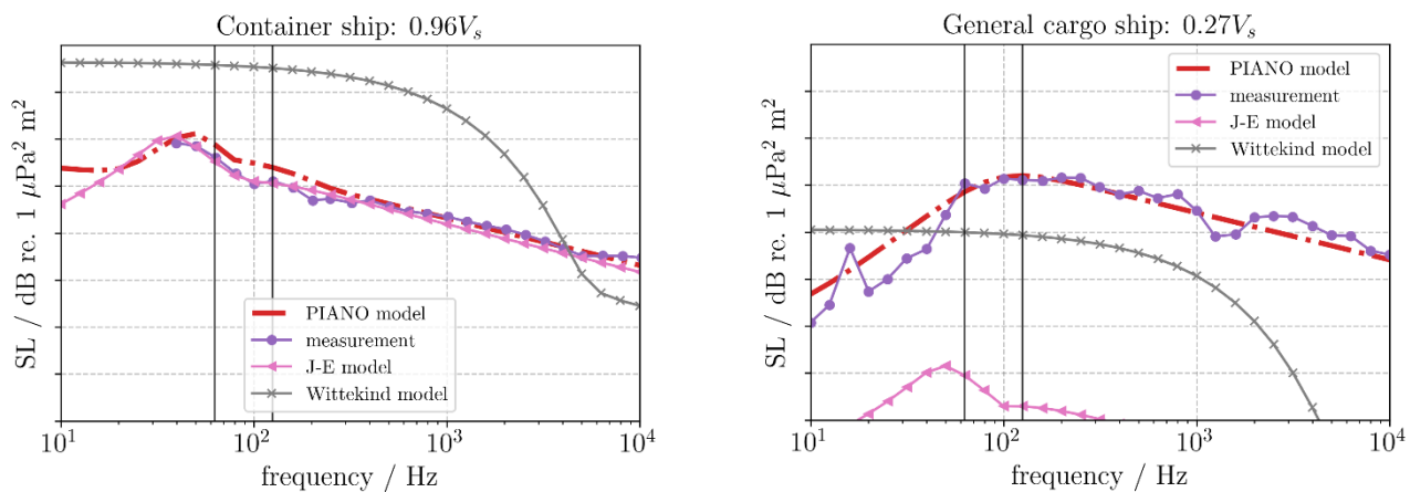
Figure 3 Example source level spectra in dB as a function of frequency in Hz for the PIANO model, compared to measured data and existing ship point source models: (left) container ship and (right) general cargo vessel. The vessel operating speed is shown in the plot titles as a decimal fraction of the service speed V_s . No scale is shown on the ordinate for confidentiality reasons relating to the measurement data. Scale divisions of the ordinate are 10 dB, such that the total y axis range is 80 dB. Measurement data made available to MARIN through the Cooperative Research Ships (CRS) framework.
