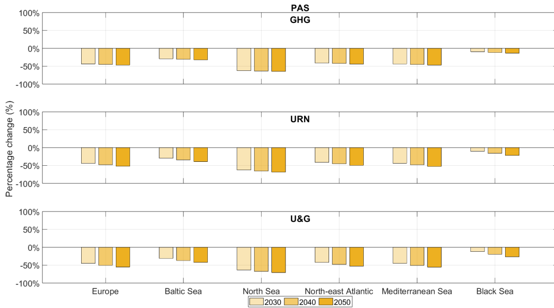
Figure 83 PAS vessel category: Comparing the percentage change in the forecast sound energy density at different regions at 63 Hz for GHG, (middle) URN, and (bottom) U&G forecast scenarios are shown in 2030, 2040, and 2050.
