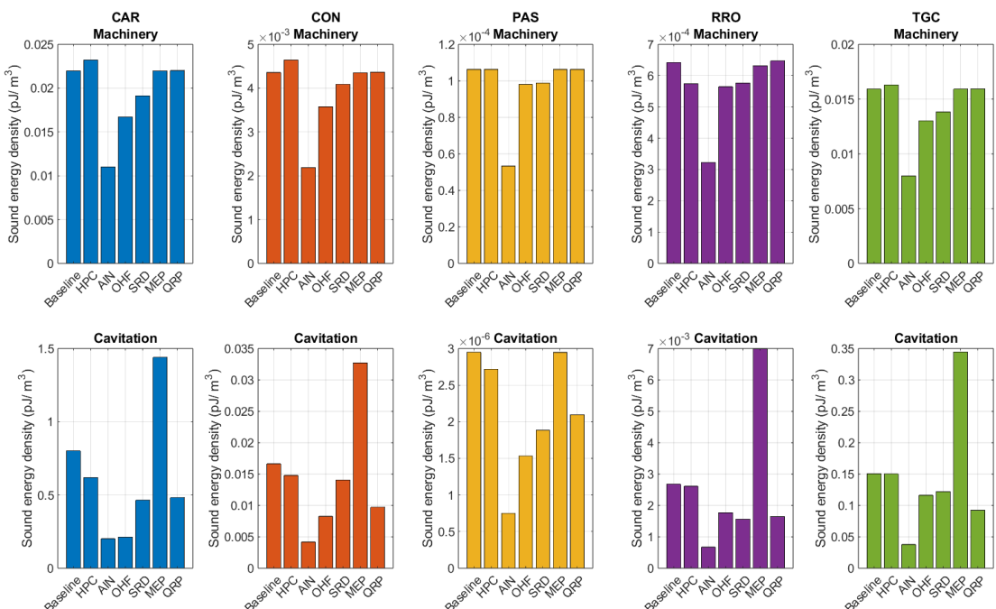
Figure 66 Black Sea: Forecast sound energy density for the 100 % penetration rates for each mitigation measure at 63 Hz. Sound energy density is calculated for (top) machinery and (bottom) cavitation components.
