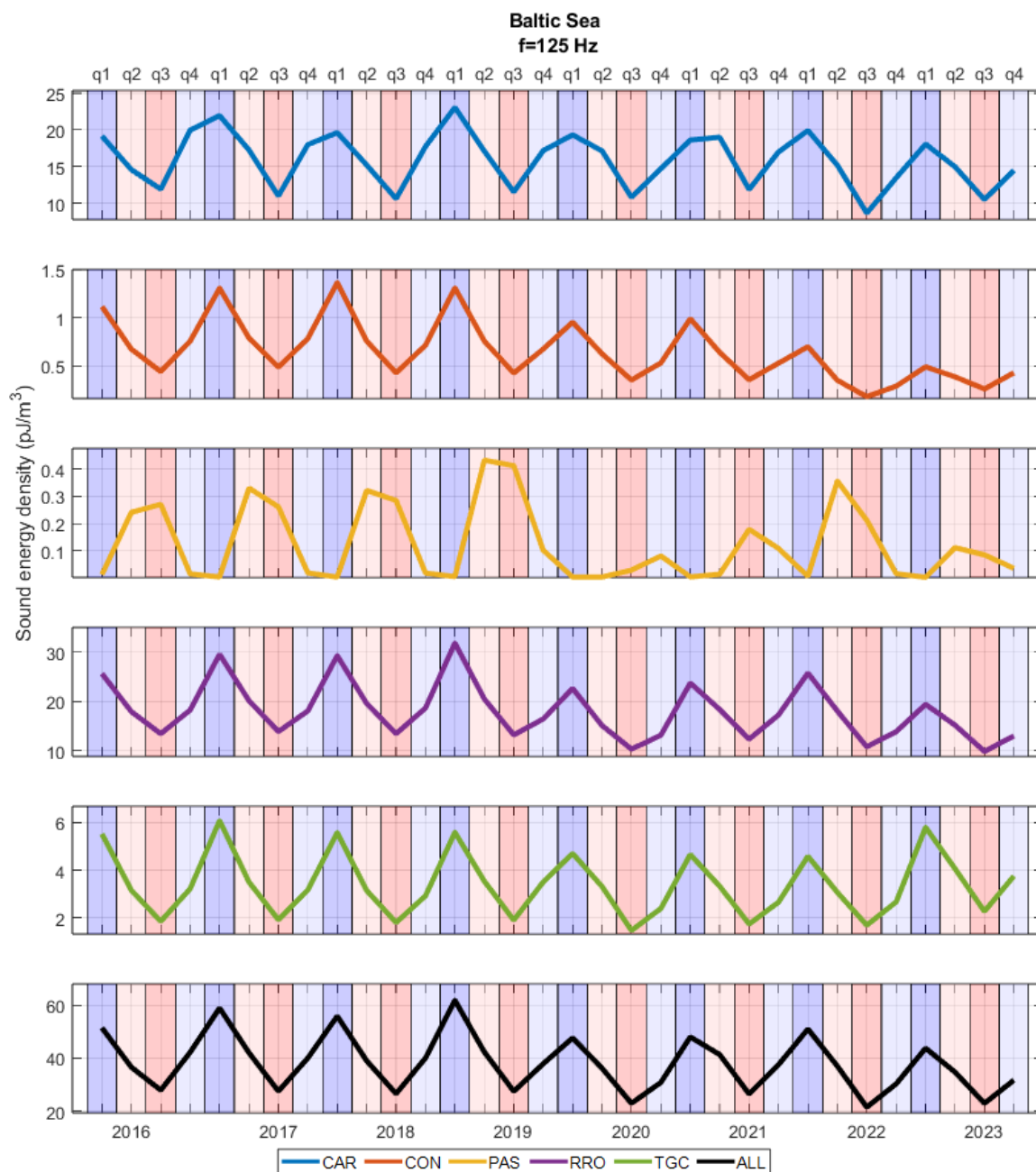
Figure 26 Baltic Sea: Sound energy density (in pJ/m 3 ) of different vessel categories for each quarter in chronological order at 125 Hz.
