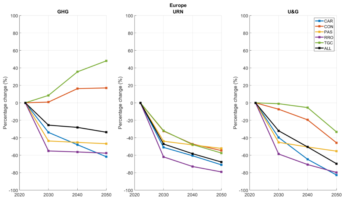
Figure 60 Europe: Forecast percentage change in the sound energy density compared to the BAU scenario at 63 Hz.
