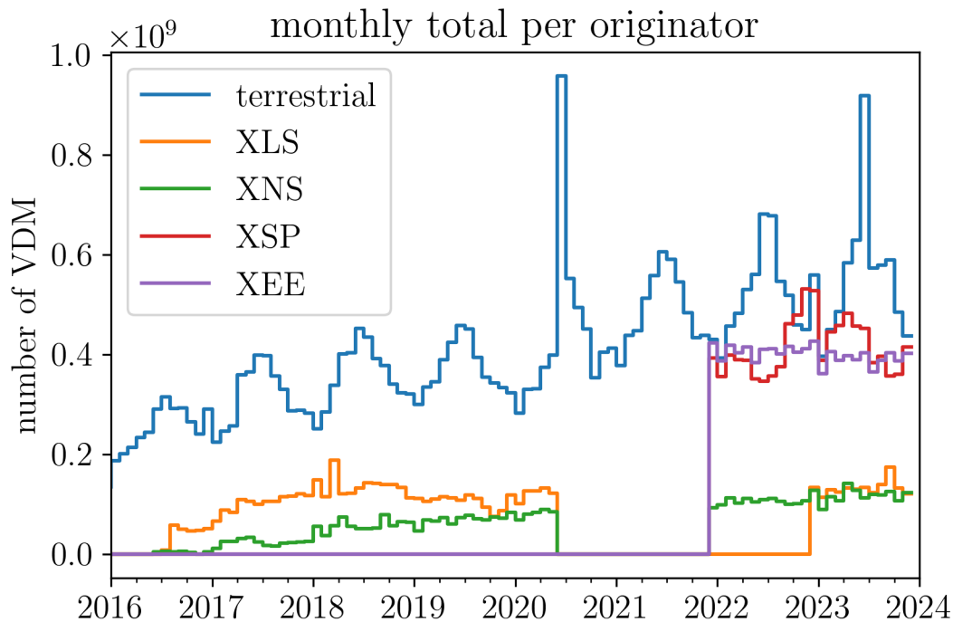
Figure 105 Monthly total Vessel Data Messages (VDM) per originator for the entire Automatic identification system (AIS) dataset used to generate the ship tracks. The terrestrial data is the sum of all messages provided by Member States' land-based receiver stations. The other originators are all satellite. NB: Number of messages does not directly correspond to the number of data points in the processed ship tracks.
