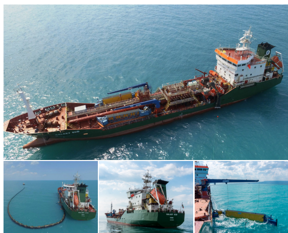
Skimmer
