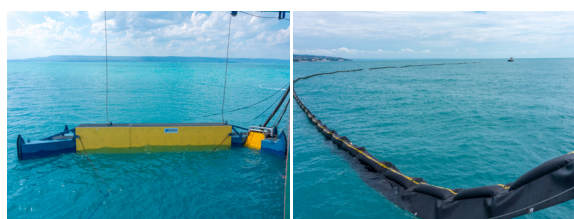
Sweeping arm
